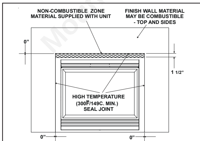
Figure 14. Sealant Material
