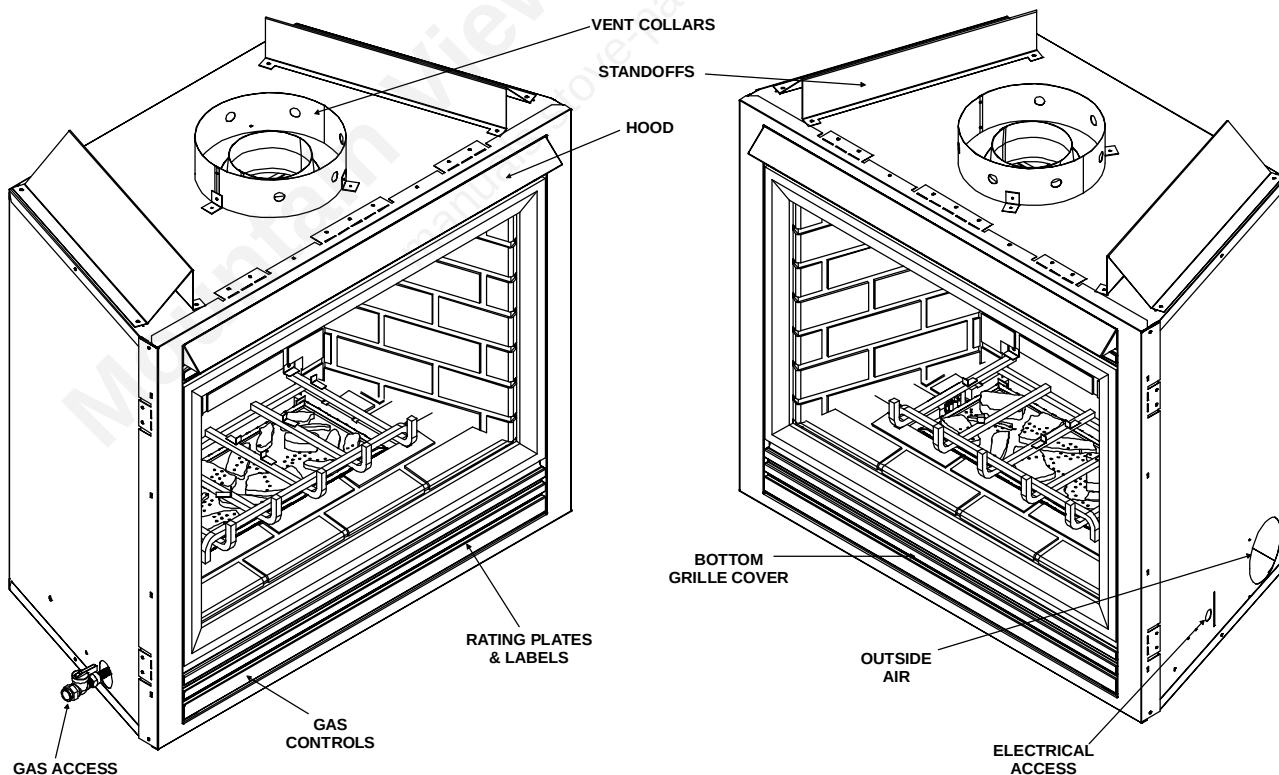
Figure 1. Diagram of the 7000TV and 6000TVB
