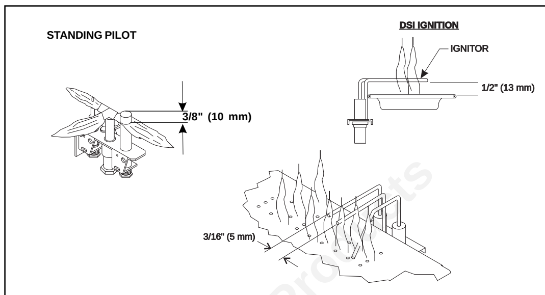
Figure 28. Gas Controls Systems
