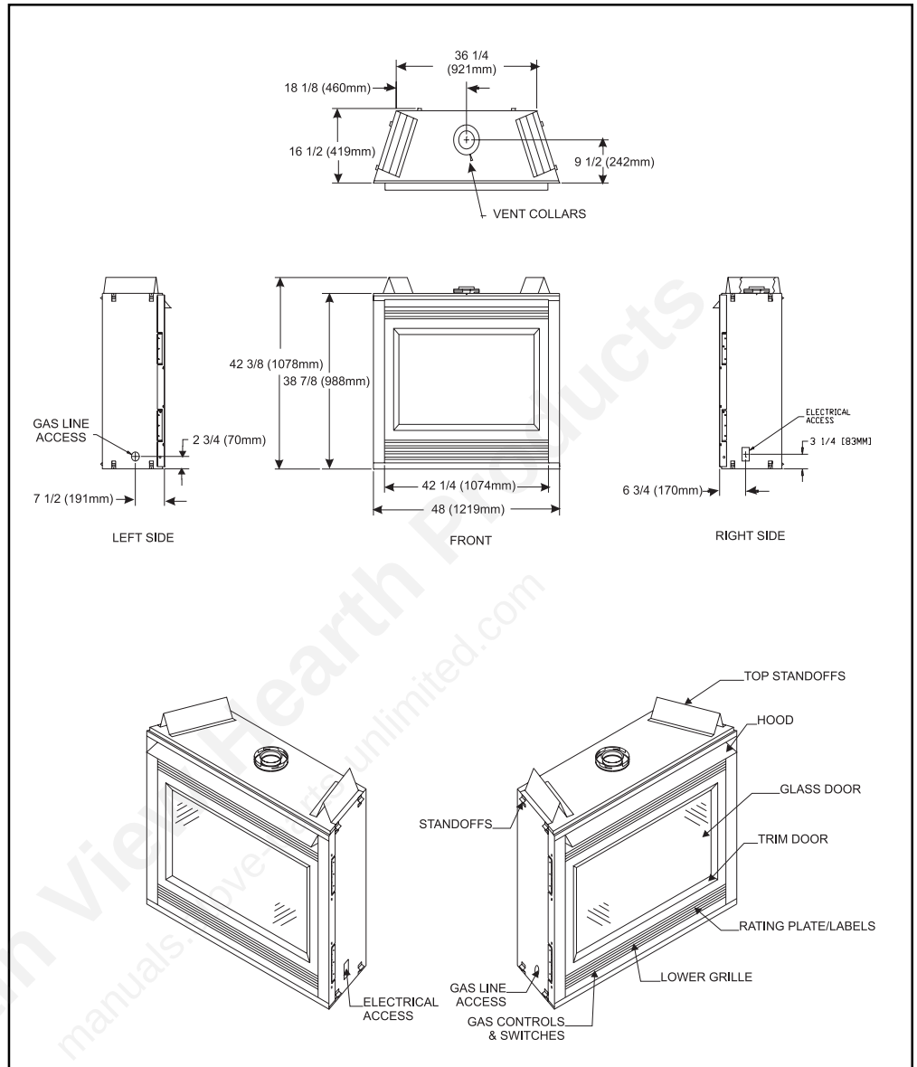
Figure 3. Diagram of SL-42DVT
