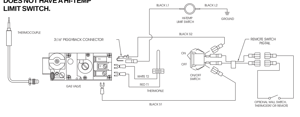
Figure 30. Standing Pilot Ignition Wiring Diagram
