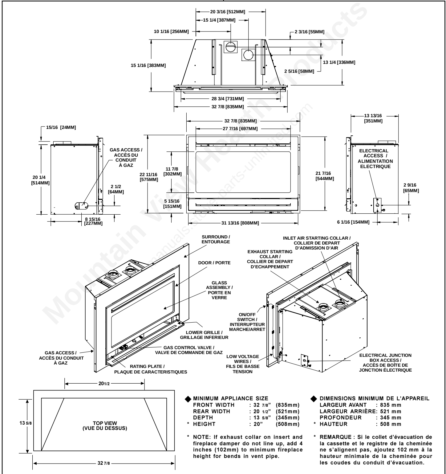
◆ Figure 1. Diagram of the AT-Supreme-D
