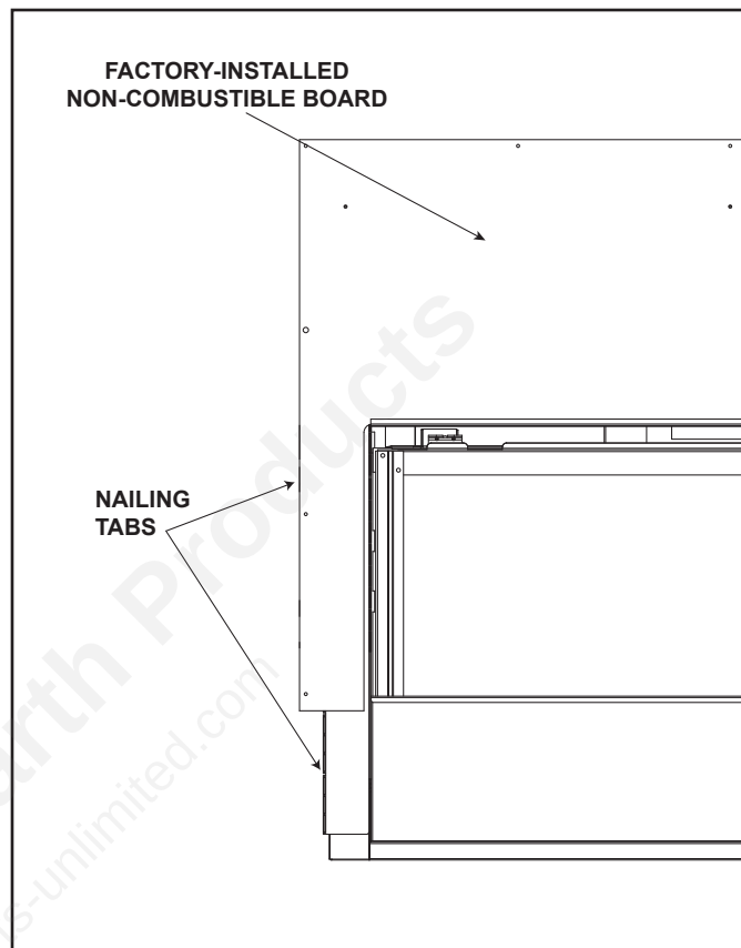
Figure 13.1 Nailing Tabs Installation Position
