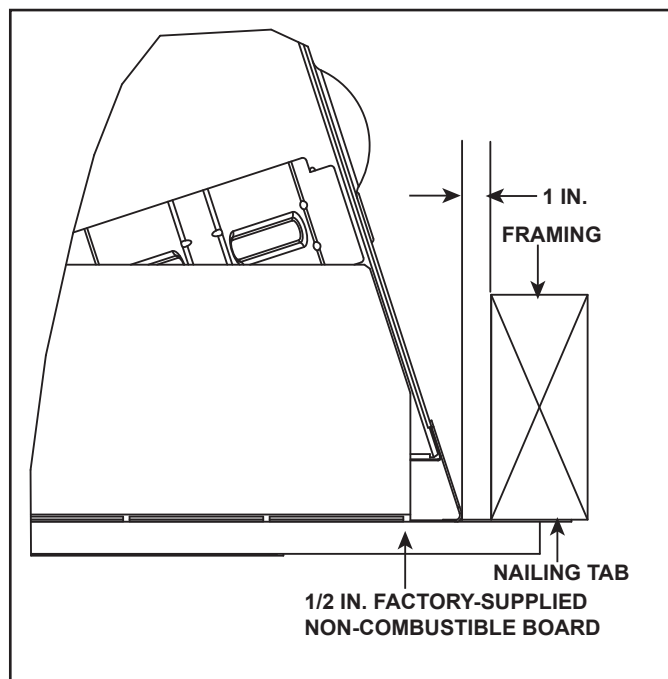
Figure 13.2 Front Side Finishing Detail
