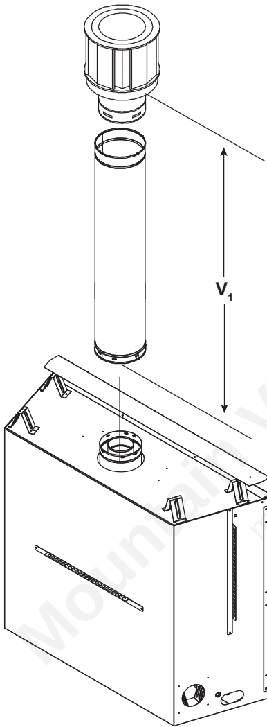
Figure 7.8 Vertical Vent Maximum
