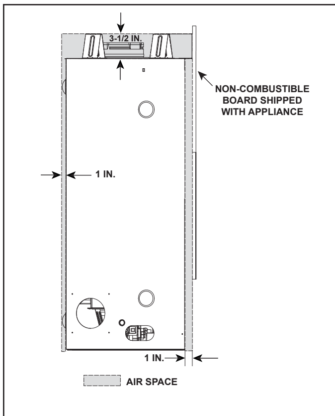
Figure 5.8 Non-Combustible Zone
