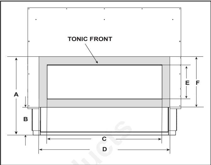
Figure 13.14 Dimensions of Tonic Decorative Front.
