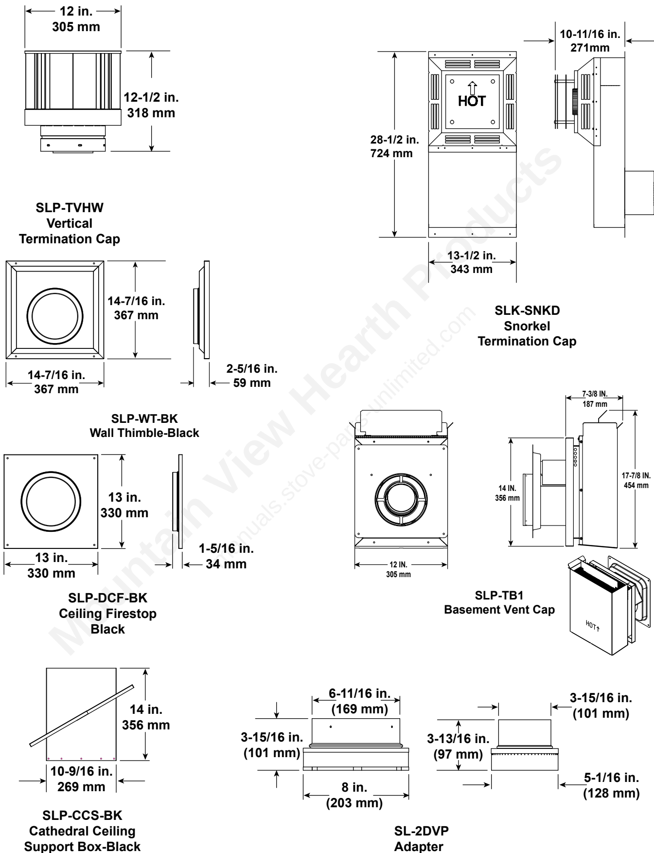
Figure 16.3 SLP Series Vent Components
