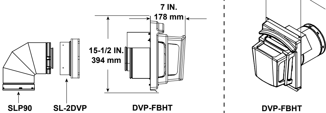
Figure 16.4 SLP Series Vent Components
