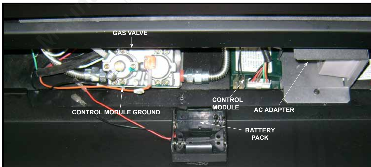
Figure 12.1 Valve Cavity
