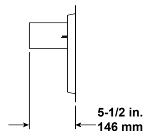
SLP-WS Wall Shield Firestop
