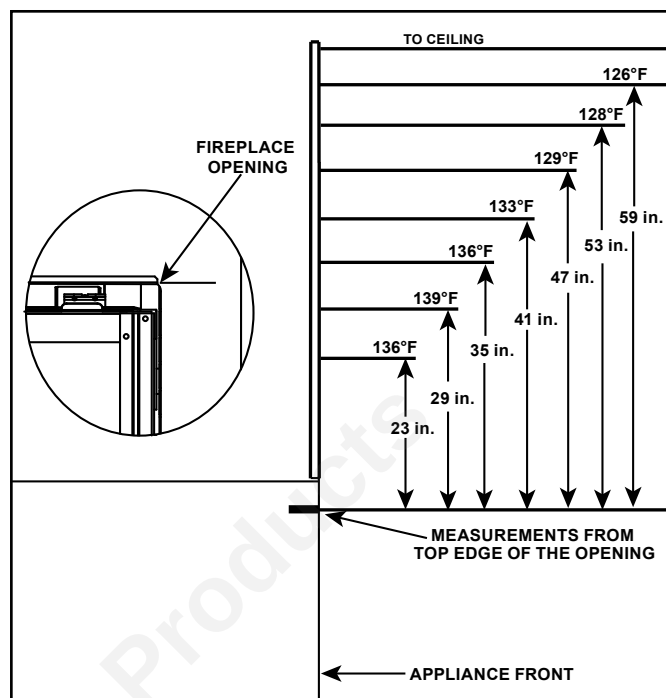
Figure 2.3. Wall Surface Temperatures Above Appliance
