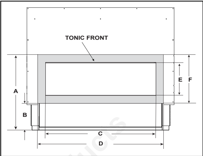
Figure 13.14 Dimensions of Tonic Decorative Front.
