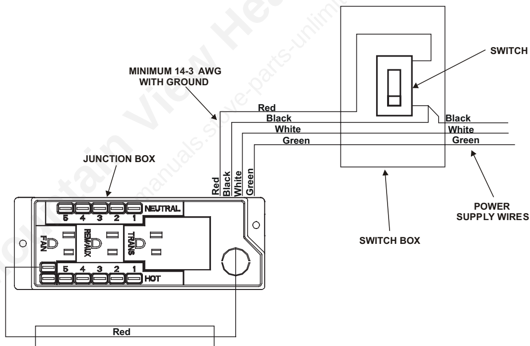
Figure 38. Junction Box Wired to Wall Switch
