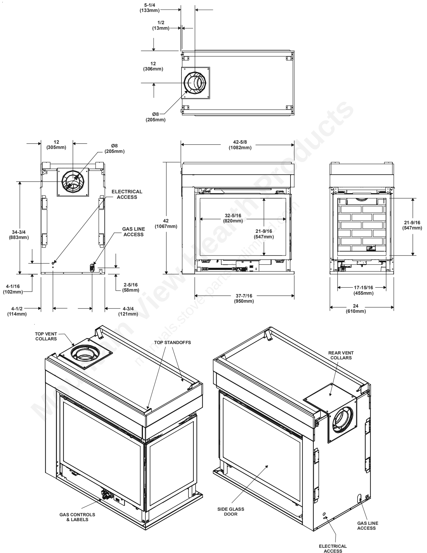
Figure 1. Diagram of the PIER-HV-IP1
