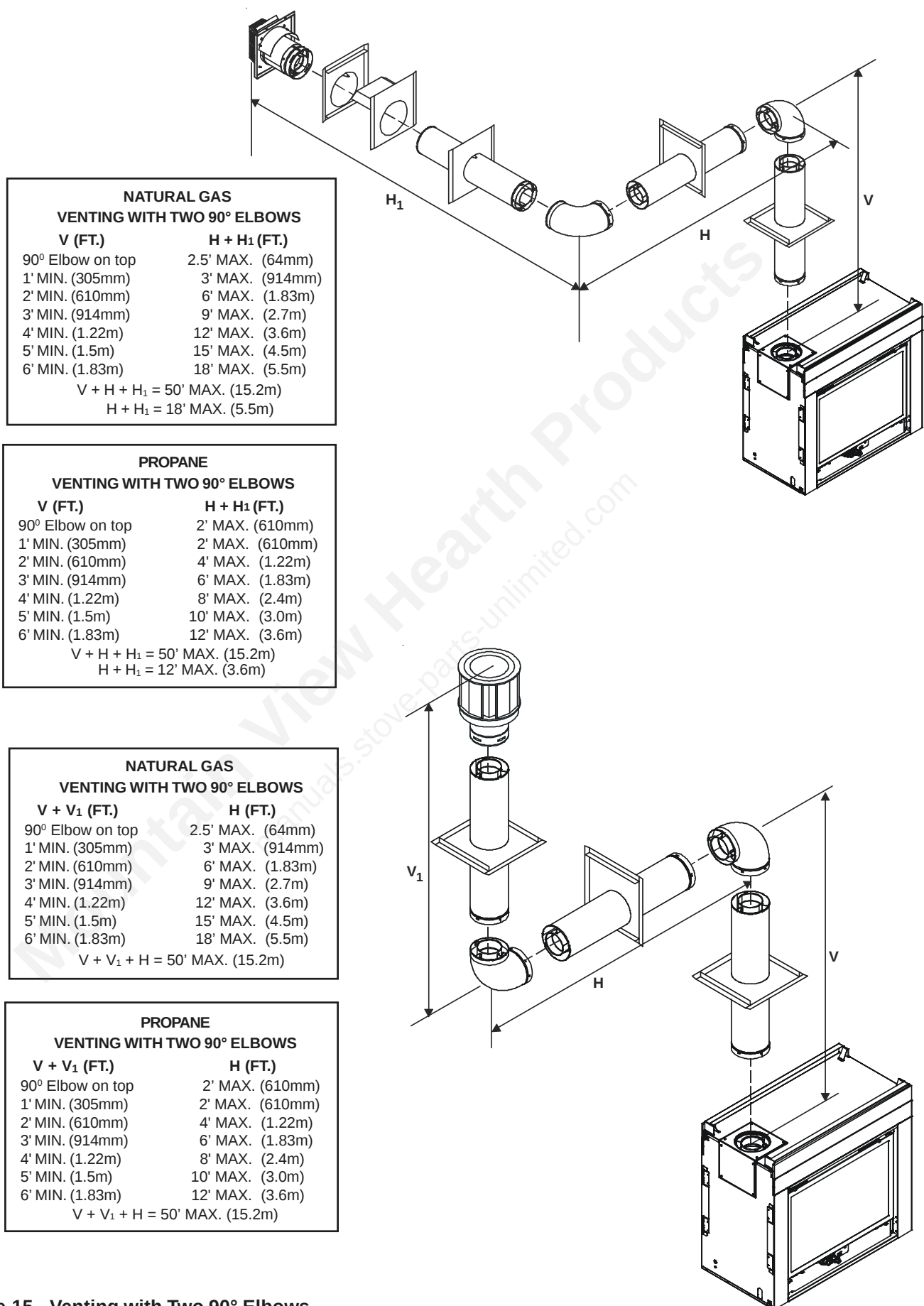
Figure 15. Venting with Two 90° Elbows
