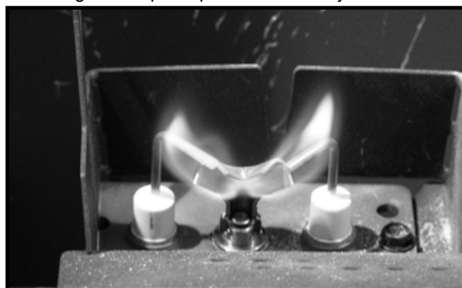
Figure 4.2 IPI Pilot Flame Pattern - Generic Pilot Bracket Shown
