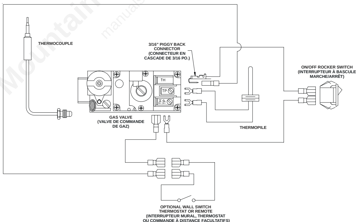
Figure 9. Standing Pilot Ignition Wiring Diagram
