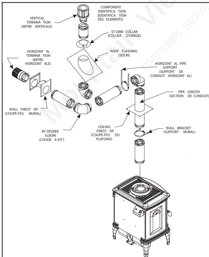
◆ Figure 4. Vent Components and Terminations
