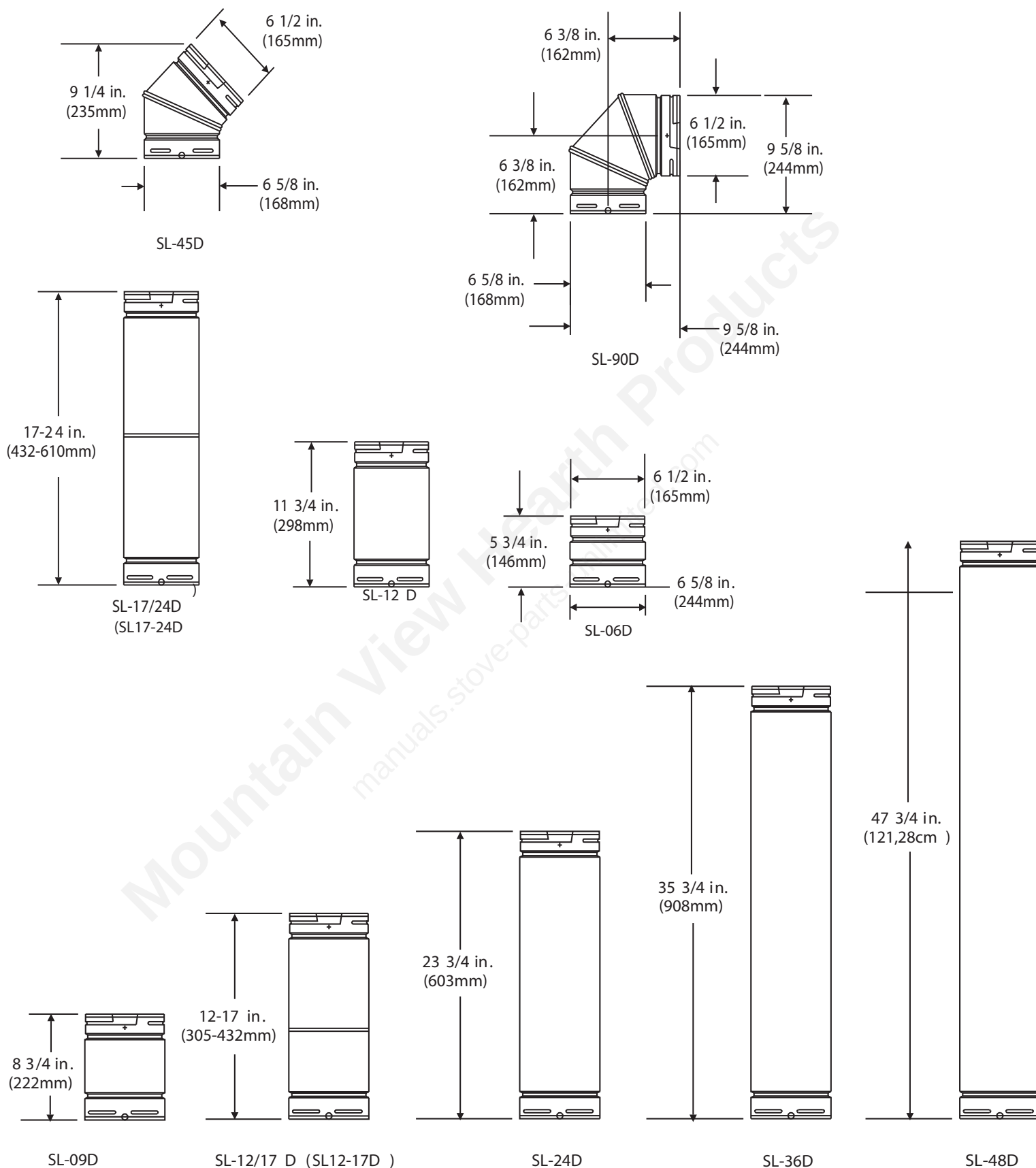
Figure 5. SL D-Series Direct Vent Component Specifications (4-inch inner pipe 6-5/8-inch outer pipe)
