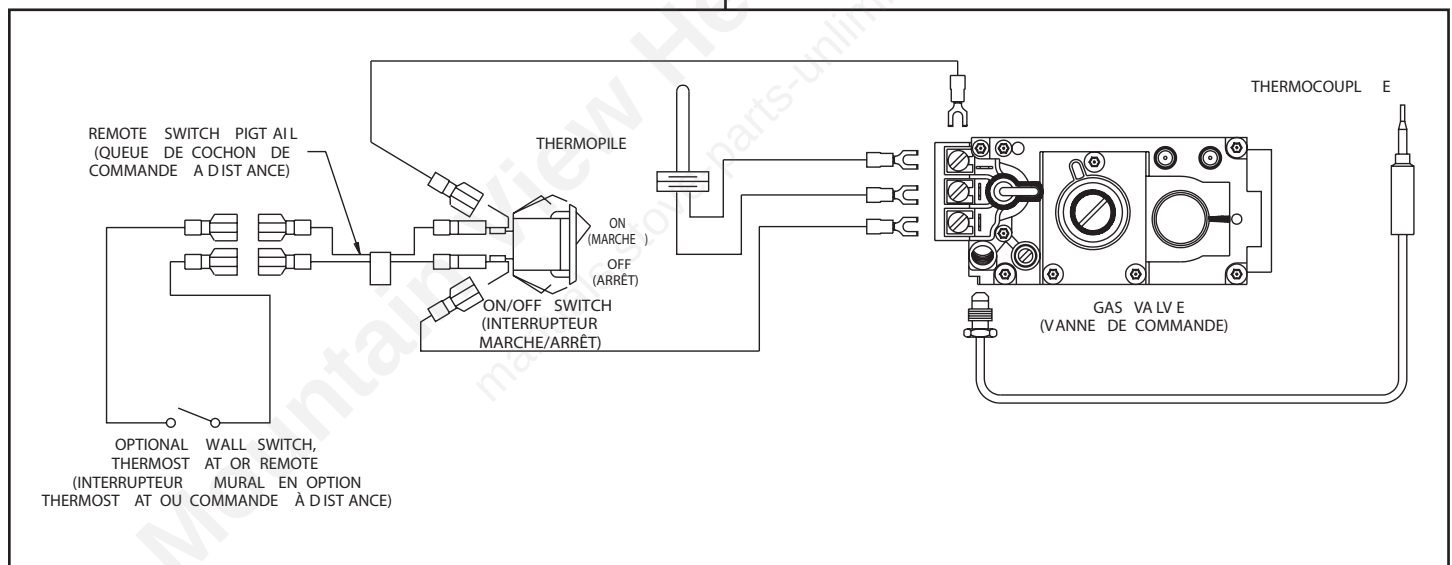
Figure 24. Standing Pilot Ignition Wiring Diagram
