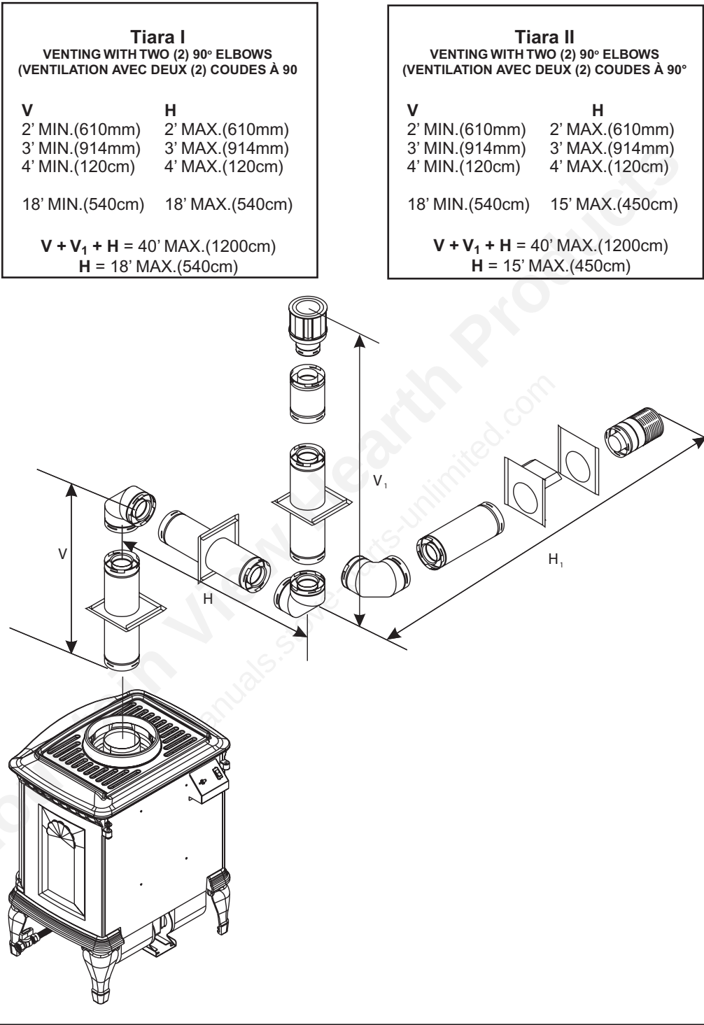
Figure 9. Vent System with Two 90° Elbows
