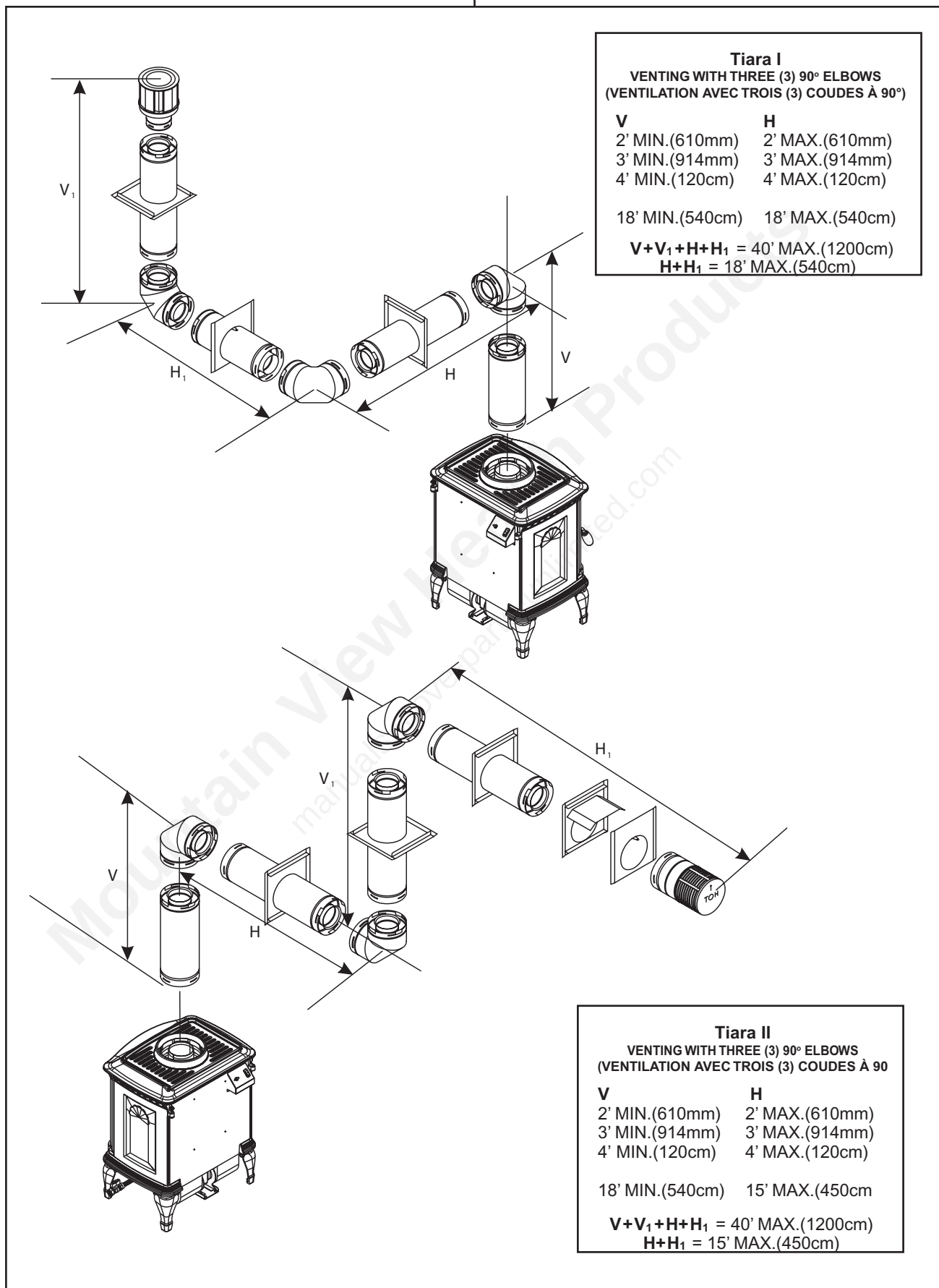
Figure 10. Vent System with three 90° elbow
