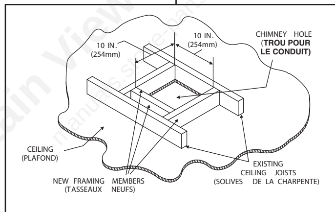
Figure 16. 10" x 10" Hole and New Framing Members
