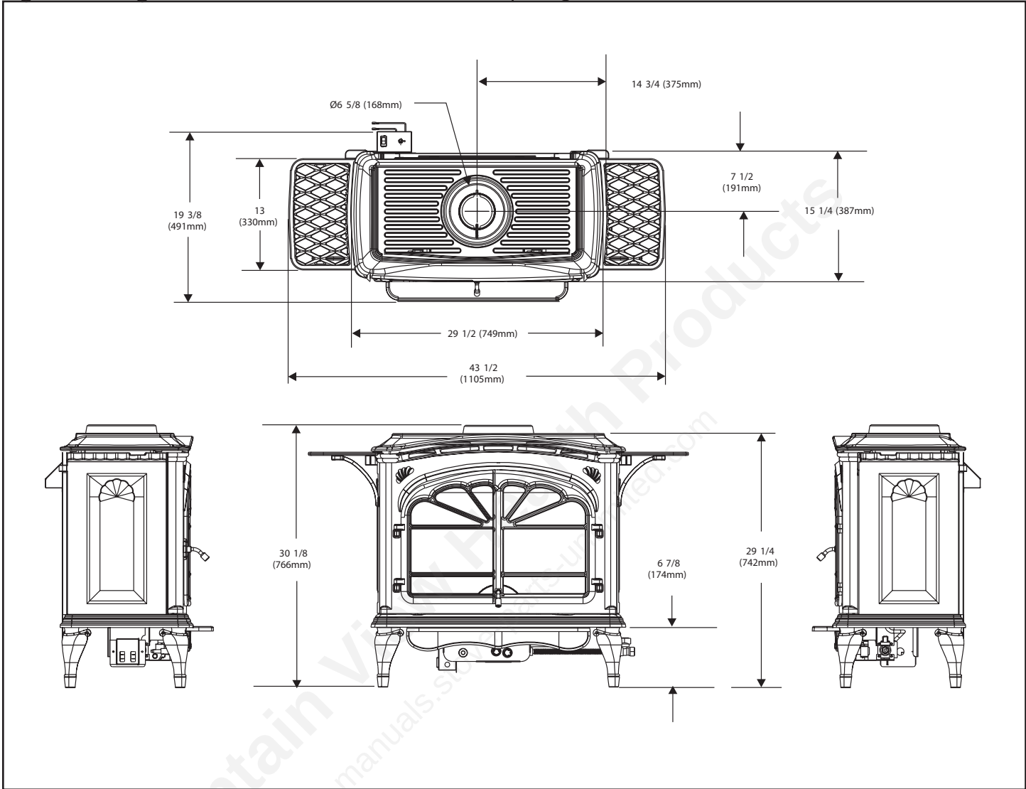
Figure 2. Diagram of the Tiara II
