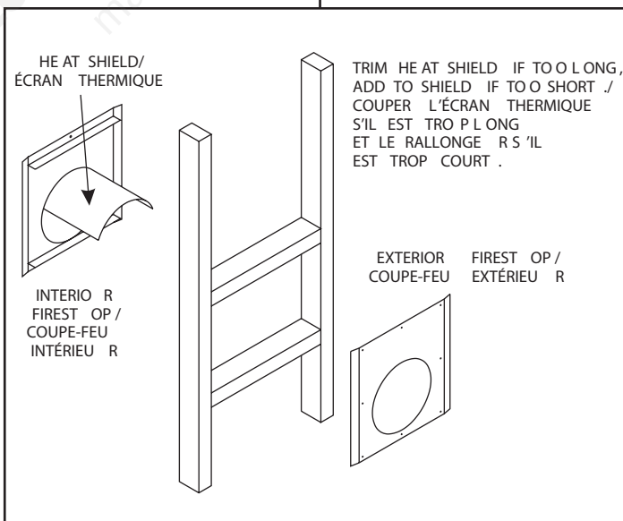
Figure 15. Heat Shield, Interior and Exterior Firestops
