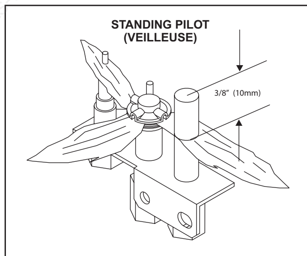
Figure 29. Pilot Flame Patterns
