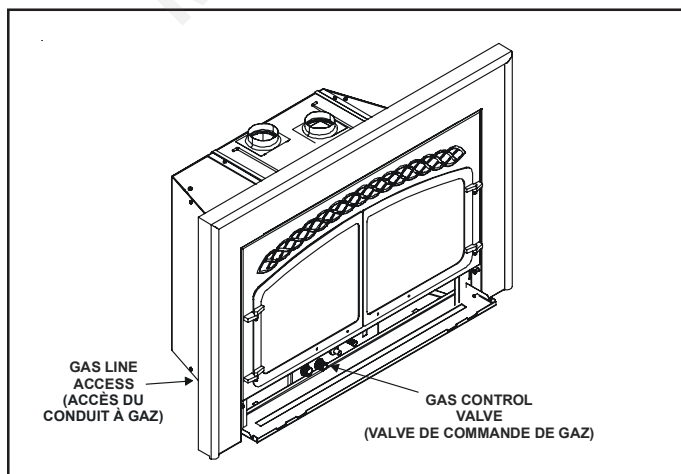
Figure 8. Gas Supply Line
