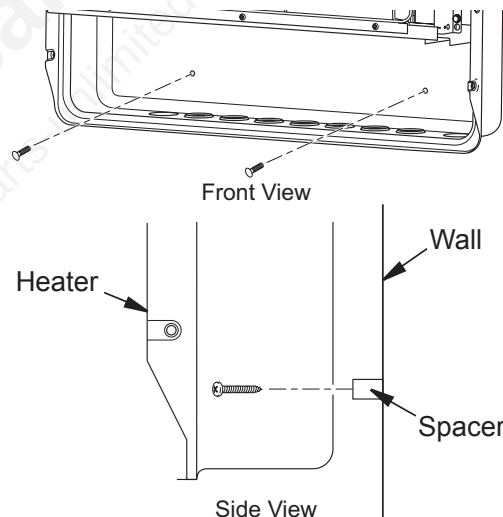
Figure 12 - Installing Bottom Mounting Screws
