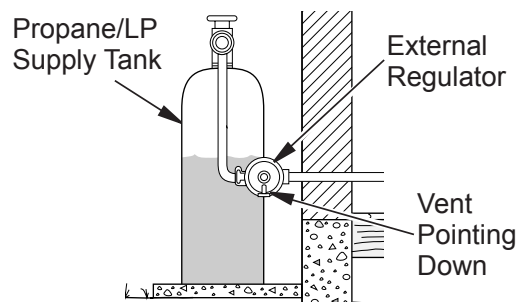
Figure 14 - External Regulator With Vent Pointing Down
