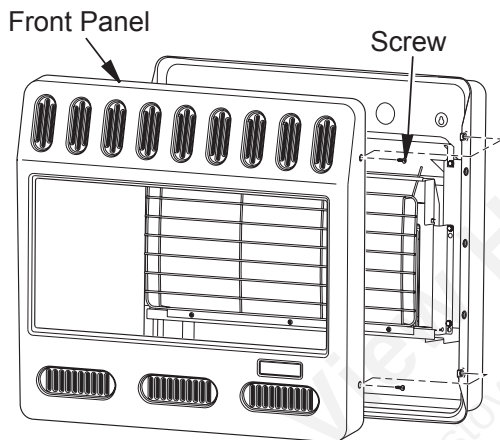
Figure 7 - Removing Front Panel Of Heater
