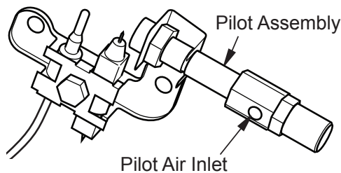
Figure 26 - Pilot Air Inlet
