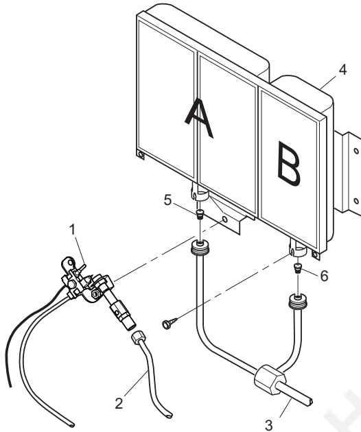
Burner Assembly LCR16PT, LCR18NT, HDR16PT and HDR18NT
