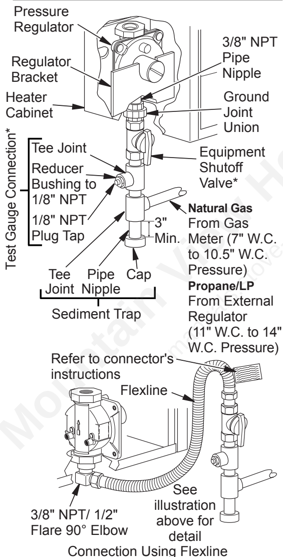
Figure 15 - Gas Connection
