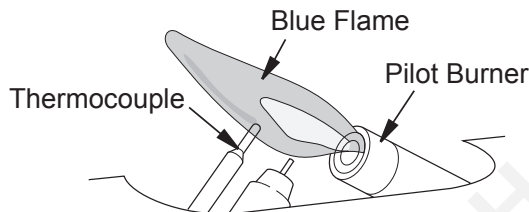
Figure 22 - Correct Pilot Flame Pattern
