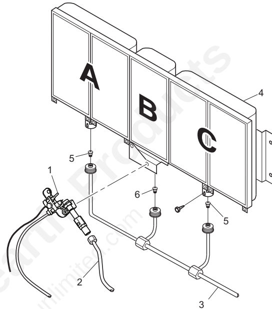
Burner Assembly LCR26PT, LCR30NT, HDR26PT and HDR30NT
