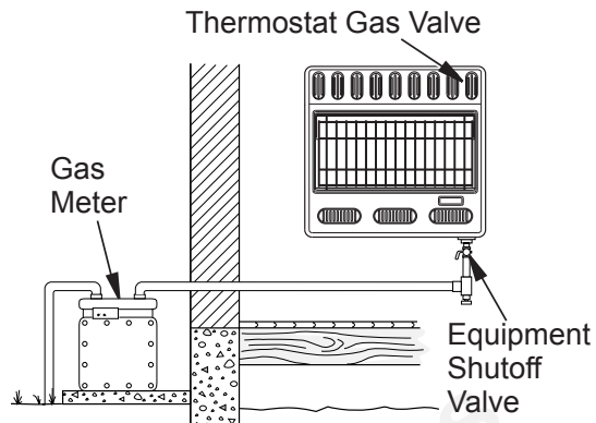
Figure 17 - Checking Gas Joints for Natural Gas
