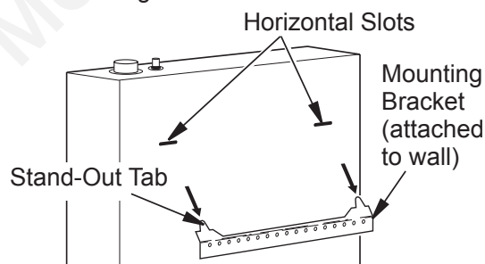
Figure 11 - Mounting Heater Onto Mounting Bracket
