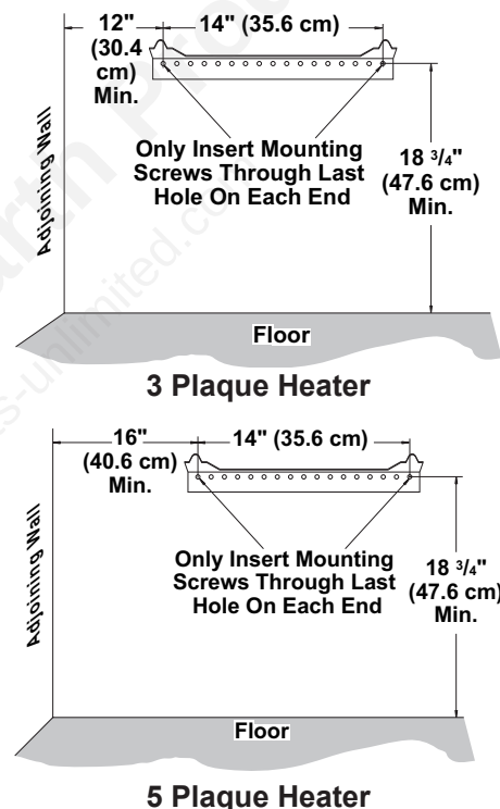
Figure 8 - Mounting Bracket Clearances
