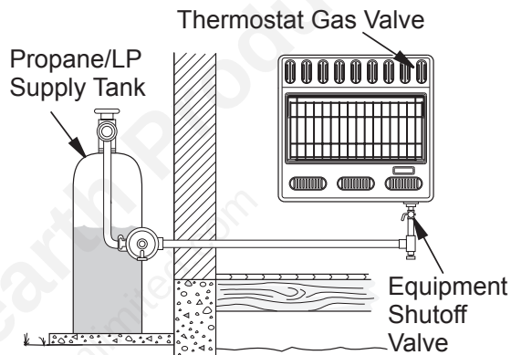
Figure 18 - Checking Gas Joints for Propane/LP Gas
