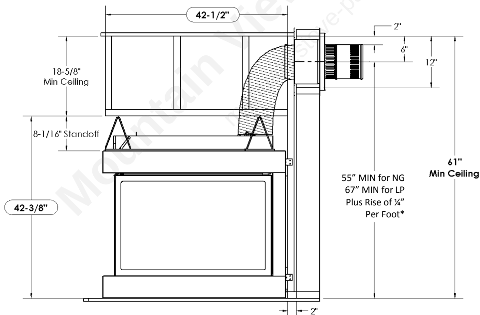
Vertical Venting MUST maintain 1" clearance to combustibles.
