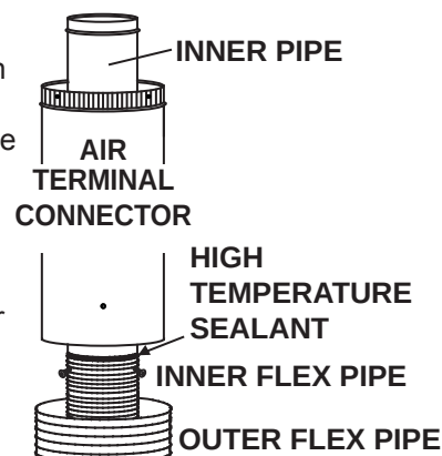
ROOF SUPPORT
