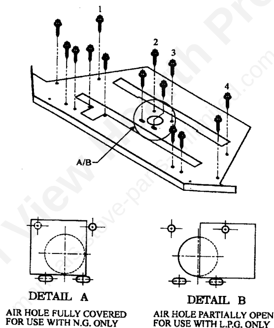
Figure 22 Firebox Bottom Removal
