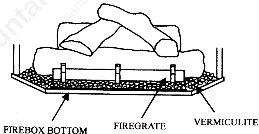
Figure 16 Installing Vermiculite
