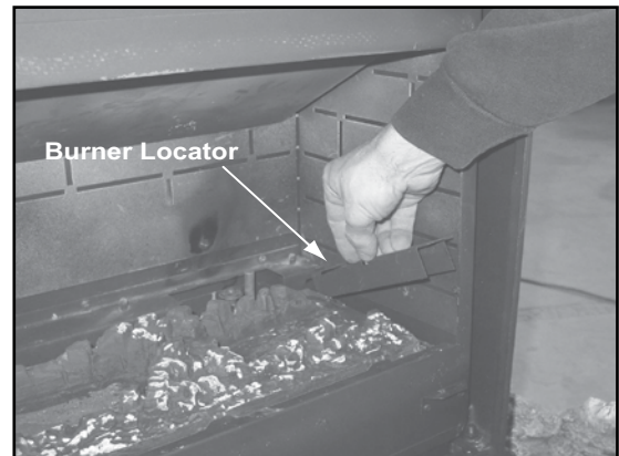
Figure 8.8 To remove the burner pan locators from the left and right sides of the burner, remove one screw from each side, lift locators up and out.
