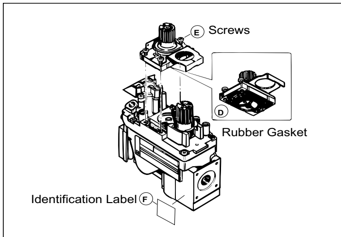
Figure 6.7 Ensure that the rubber gasket (D) is properly positioned and install the new HI/LO pressure regulator assembly to the valve using the new screws (E) supplied with the kit. Tighten screws securely. (Reference torque = 25 in./lb.) Install the enclosed identification label (F) to the valve body where it can be seen.
