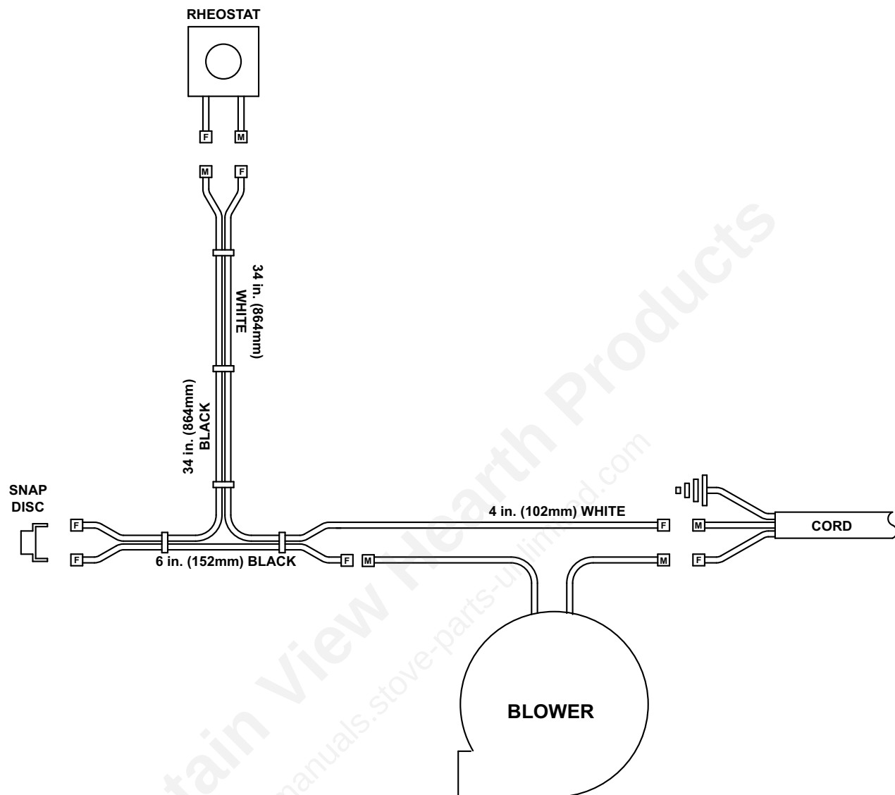
Figure 8.26 Blower Wiring Diagram
