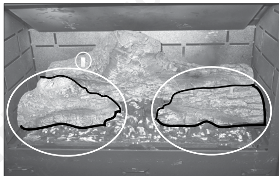
Figure 8.20 Set left and right partial logs (with butt end towards the side of the appliance firebox) in the grooves provided on the burner surface.
