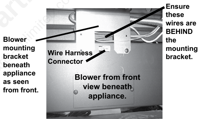
Figure 8.23 Beneath the appliance from its front side, ensure that all wiring is moved behind the blower mounting bracket which already comes installed on the bottom of the appliance. Complete blower mounting by inserting two screws through the blower into the mounting bracket. Make the wire harness connection.
