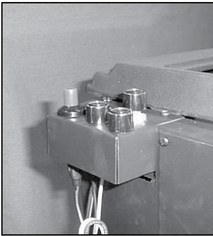
Figure 8.25 Insert the rheostat control into its opening from beneath the control panel. Fit the rheostat nut on top and tighten the nut using an 11/16 in. wrench. Attach the black knob.
