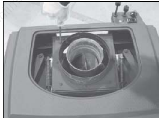
Figure 8.3 Lift out the cast insert piece on top of the appliance.
