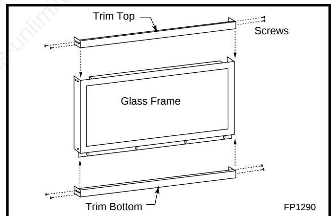
Fig. 57 Install top and bottom brass trim.
