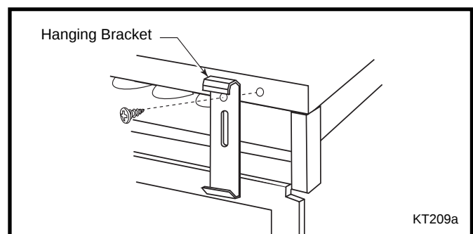
Fig. 33 Hanging bracket alignment.
