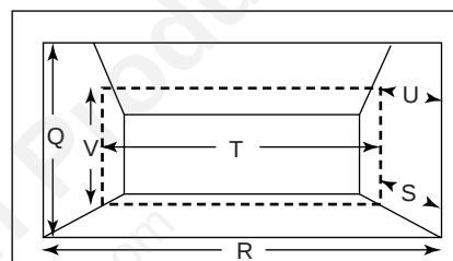
Minimum Fireplace Insert Opening
