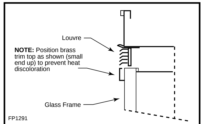
Fig. 58 Position brass trim top with small end up.
