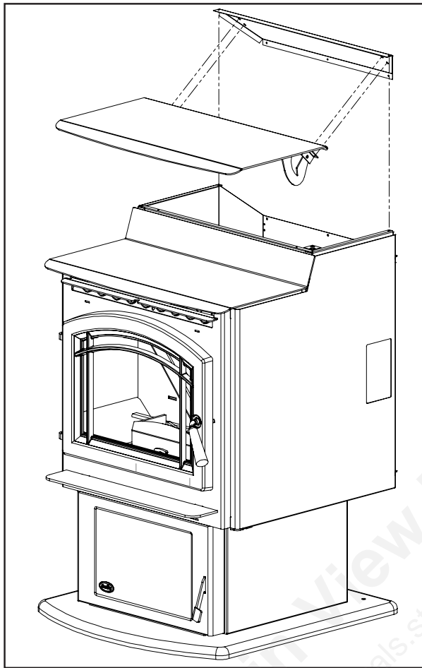
Figure 1: Removing the hopper lid and back top.
