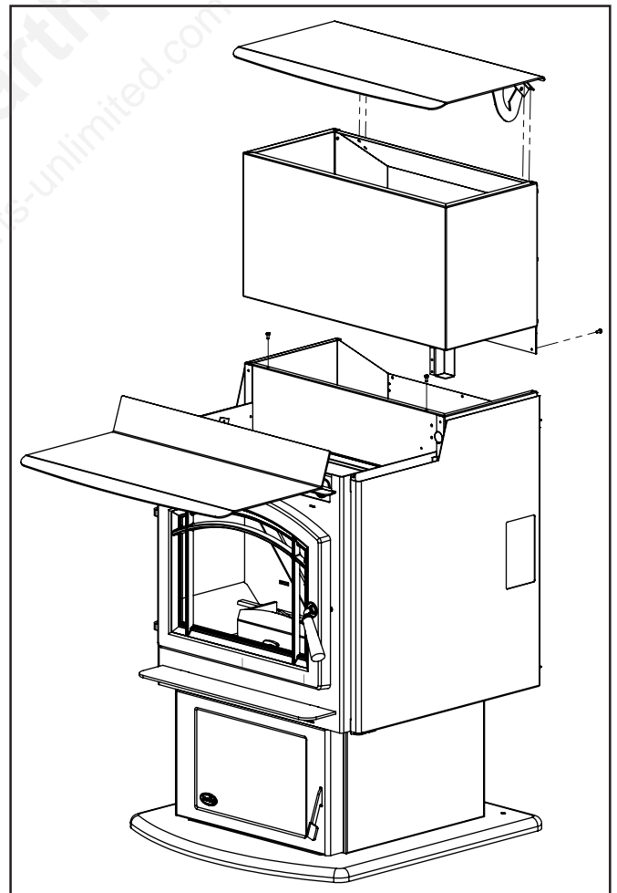
Figure 2: Installing Hopper Extension Kit.
