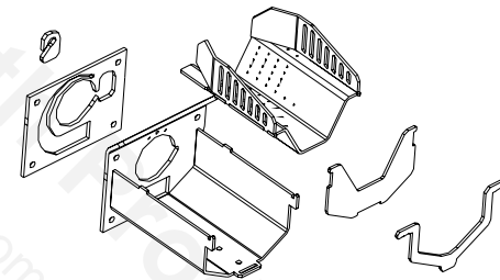
BURNPOT PELLET
