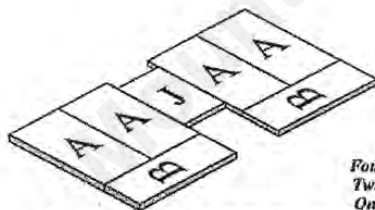
Figure 14a - Step 1, Bottom Firebrick Arrangement
