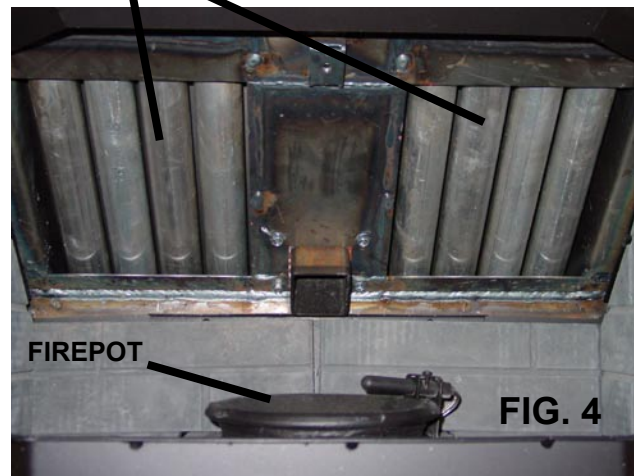
FIREBOX AREA w/ BAFFLE PLATES REMOVED
