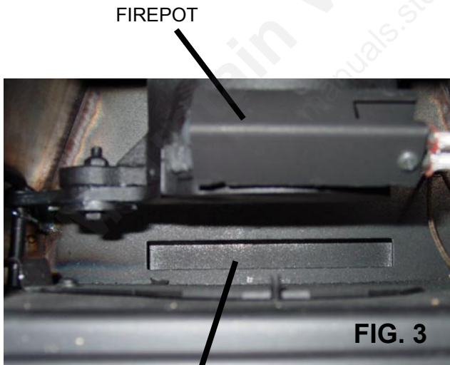
AIR INTAKE IN THE COMBUSTION CHAMBER
