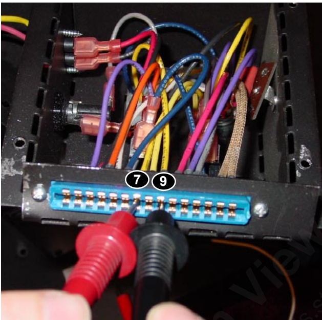
TESTING FOR CONTINUITY ON PIN 7 & PIN 9 IN THE JUNCTION BOX.
