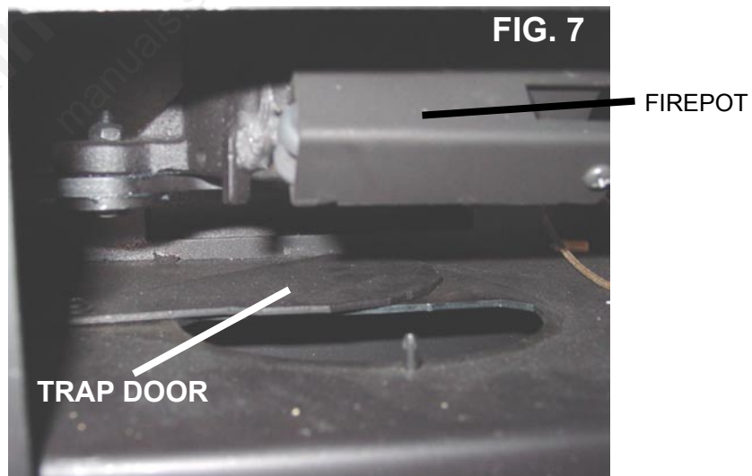
COMBUSTION AIR TRAP DOOR IN THE OPEN POSITION
