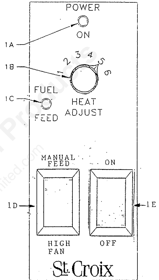
Figure 1. Control Box
