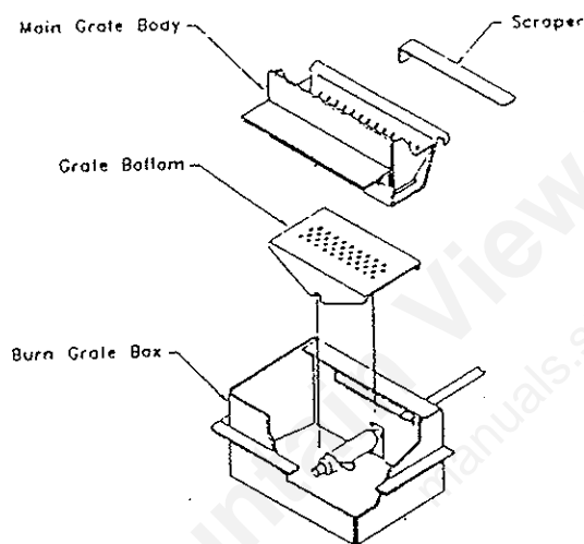
Figure 3. Self-Cleaning Grate
