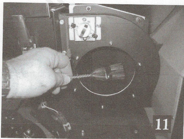
11 Clean blower housing
