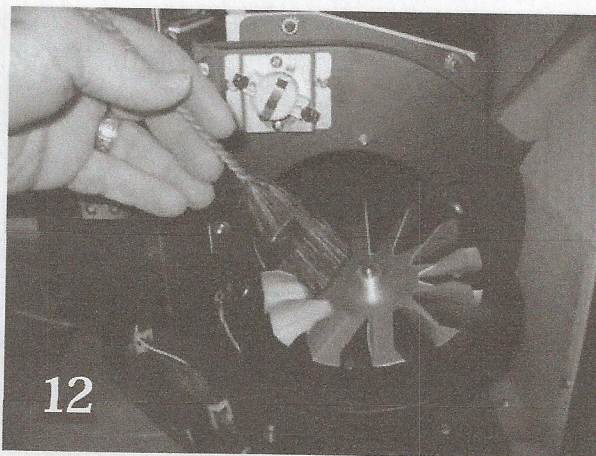
12 Clean impeller blades
