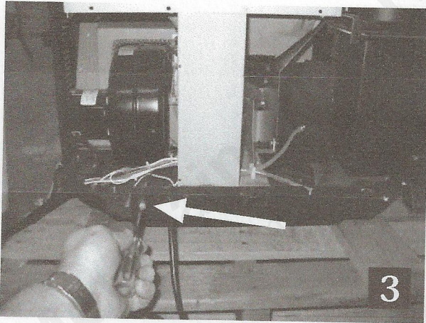
Main fuse (6 AMP quick blow) on back of pellet appliance
