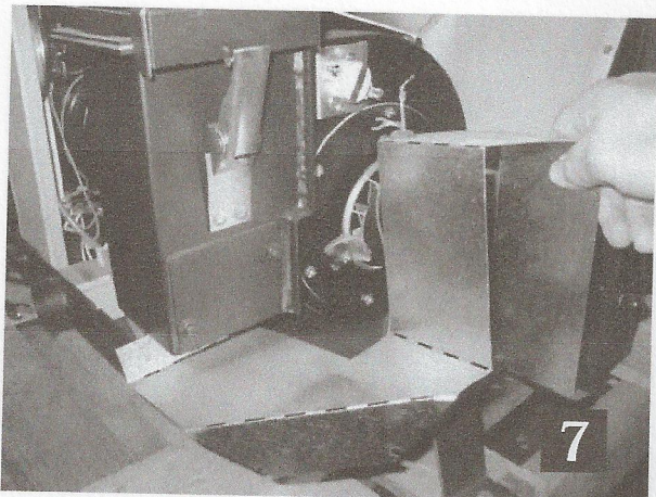
7 Remove blower heat shield (large inserts)
