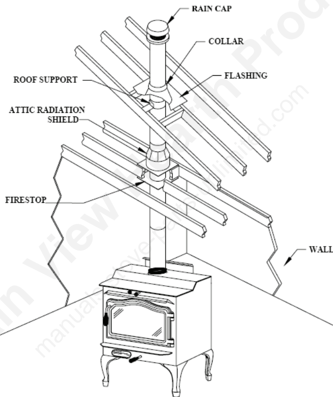
FIGURE 29: FREESTANDING PREFABRICATED CHIMNEY SYSTEM (no chase)
