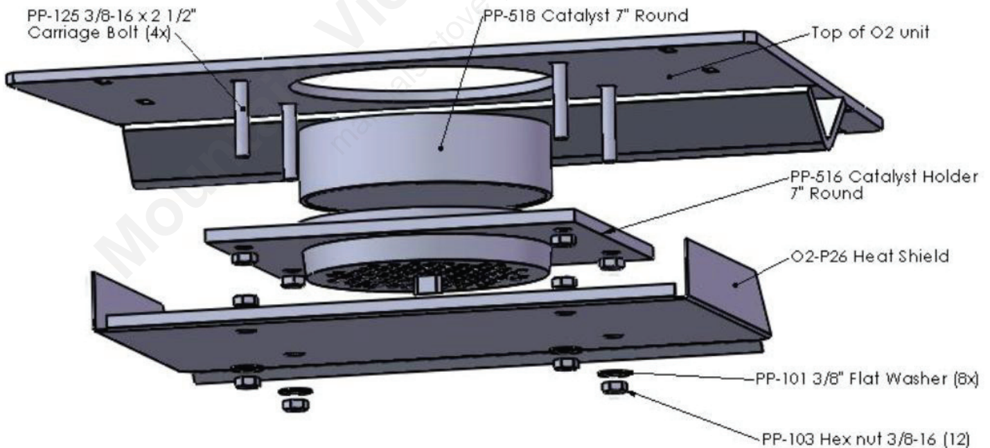
FIGURE 20: CATALYTIC SYSTEM FOR MODEL O2 STOVE
