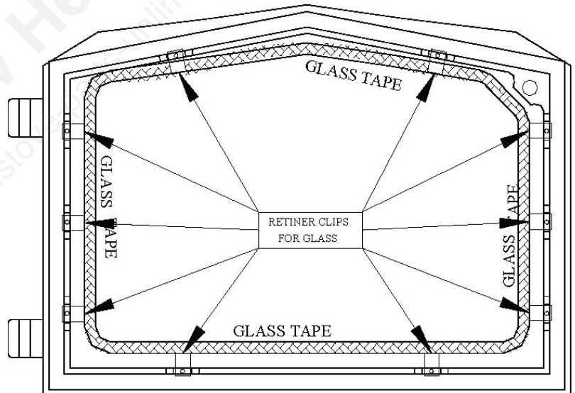
FIGURE 18: DOOR GLASS REPLACEMENT
