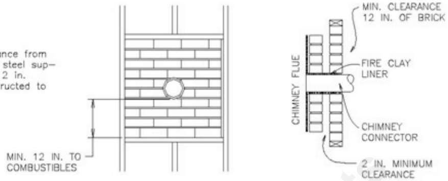
FIGURE 31: MASONRY CHIMNEY TO COMBUSTIBLE WALL
