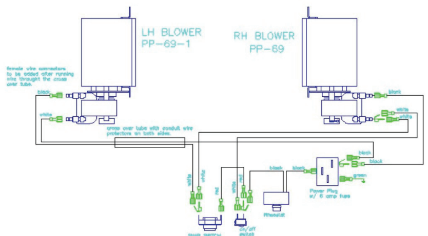
FIGURE 22: MODEL O2 BLOWER SYSTEM ELECTRICAL DIAGRAM
