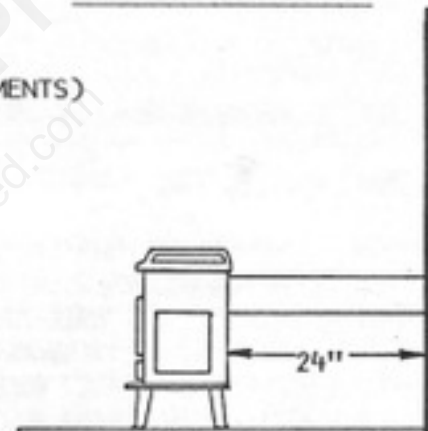
BACKWALL CLEARANCES WITH REAR FLUE CONNECTION
