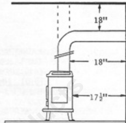
BACKWALL CLEARANCES WITH TOP FLUE CONNECTION
