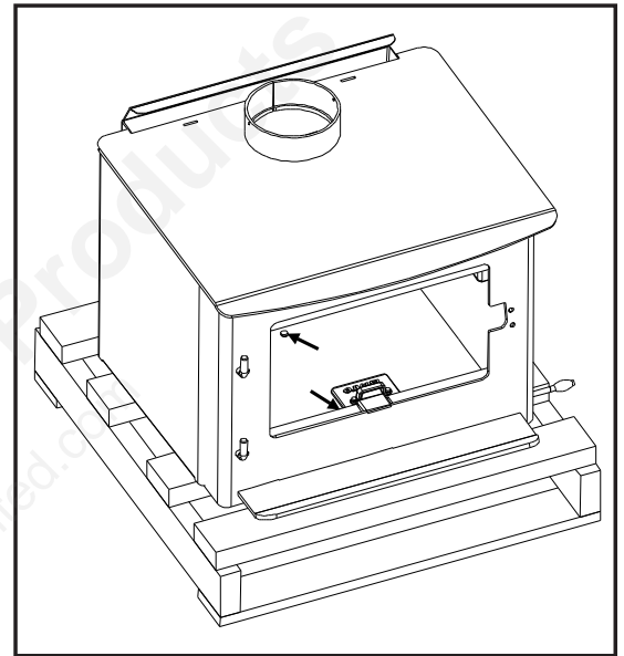
Figure 14: Bolts to remove.
