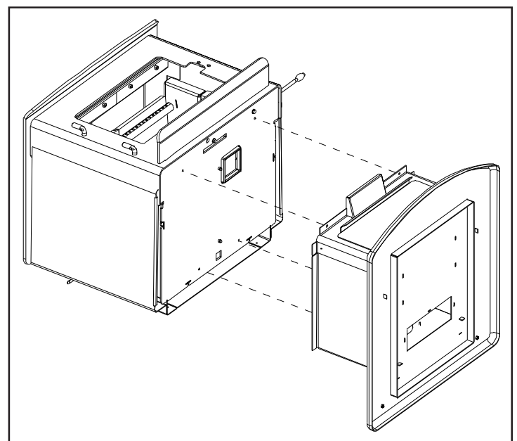
Figure 15: Installing Pedestal.
