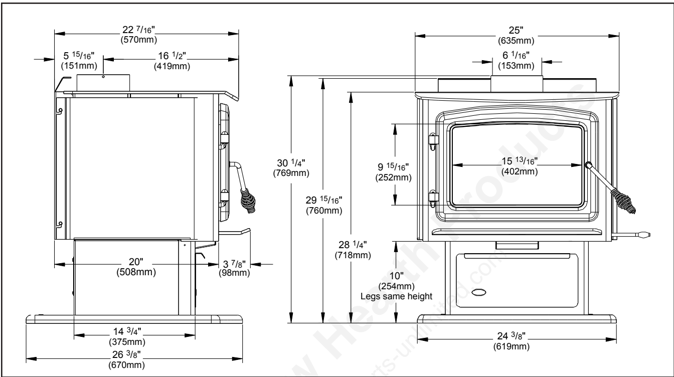
Figure 7: 1200 Freestanding Flat Top Dimensions.
