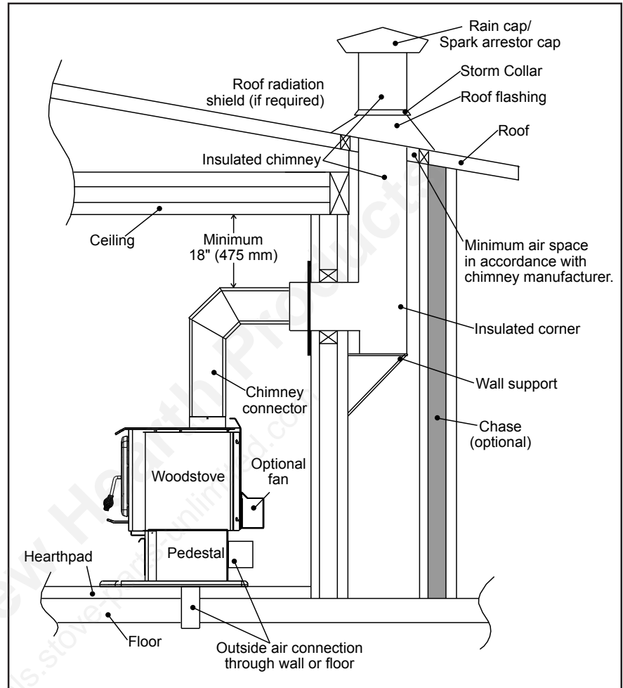
Figure 27: Standard Horizontal Installation.
