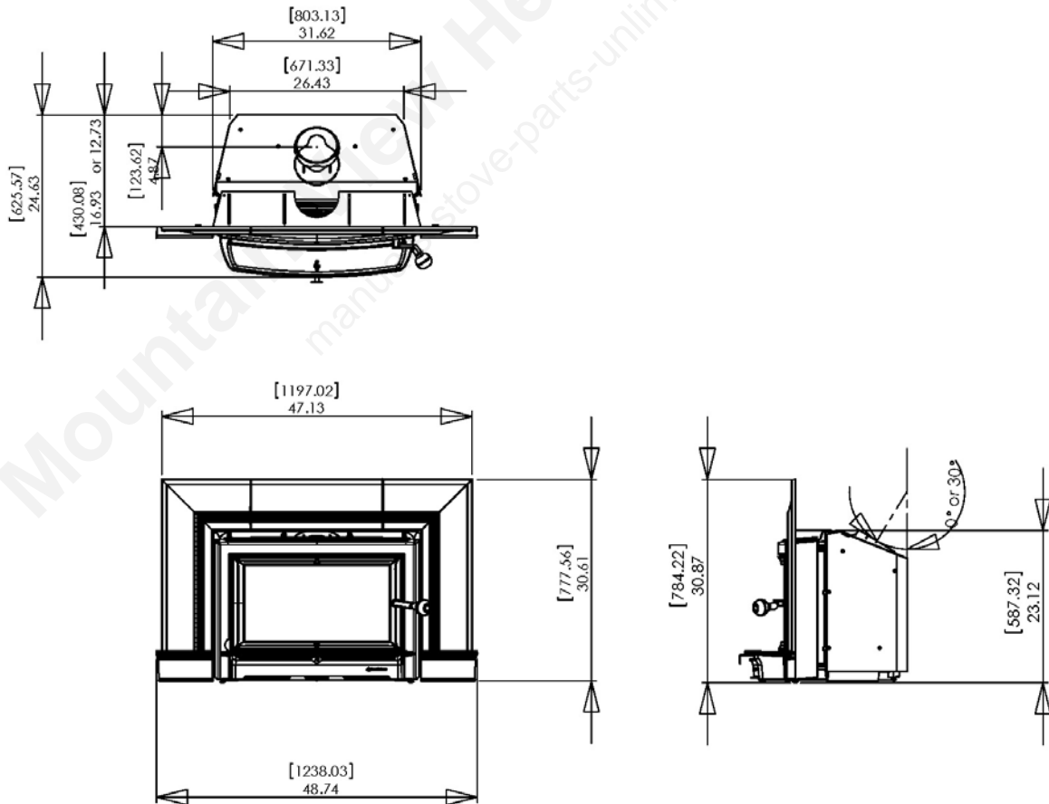
Figure 1 – Clydesdale Dimensions
