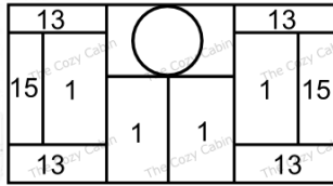
TOP VIEW - ROUND COLLAR OR COVER PLATE
