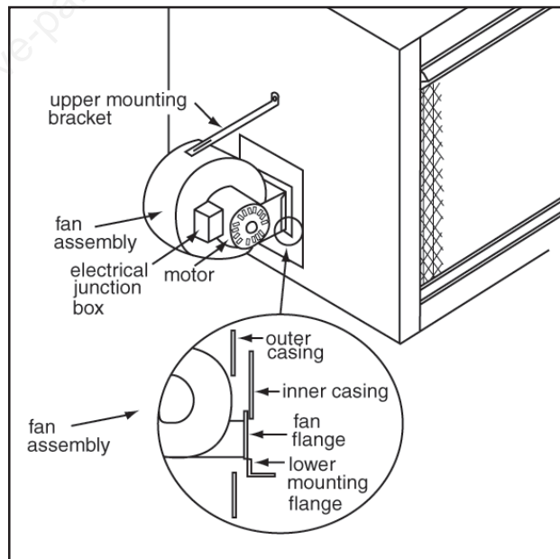
Figure 15 - Fan Mount
