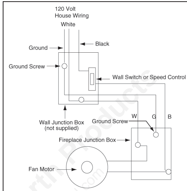
Figure 14 - Blower Wiring
