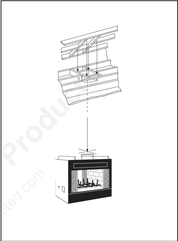
Figure 12 - Ceiling/Attic Construction
