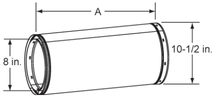
Chimney Sections
