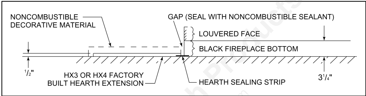
Figure 17 - Factory Built Hearth Extension
