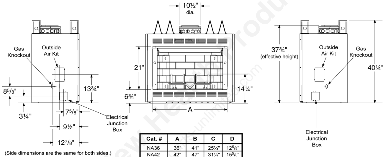
Fireplace Dimensions
