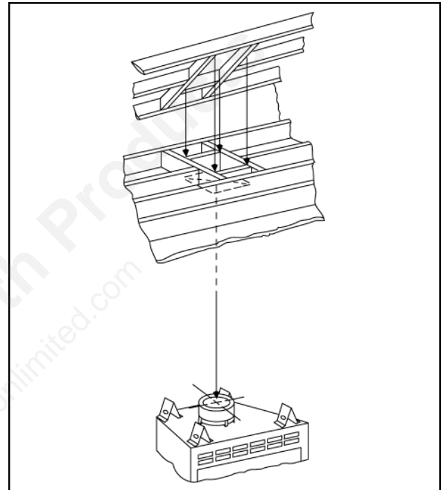
Figure 14 - Ceiling/Attic Construction
