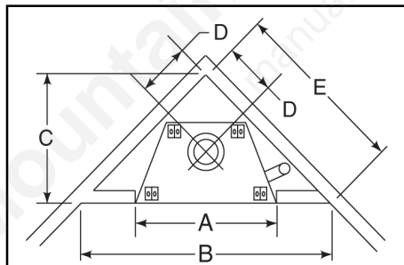
Figure 4 - Corner Installation
