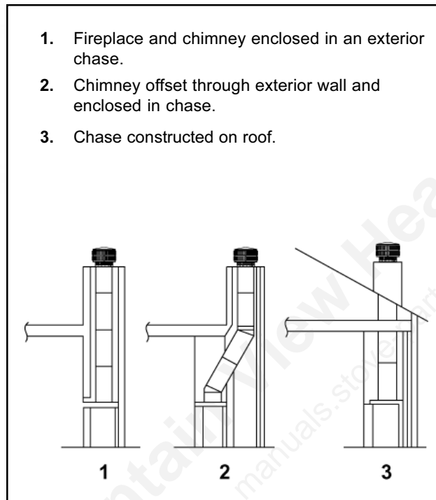
Figure 20 - Chase Constructions
