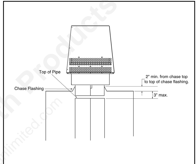
Figure 25 - Installing a TS345/TS345P Square Termination Cap
