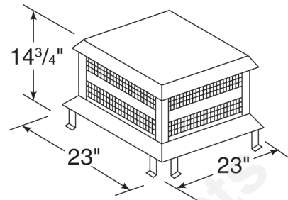
ST375 Square Termination Cap
