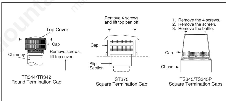
Figure 28 Chimney & Termination Cap Cleaning
