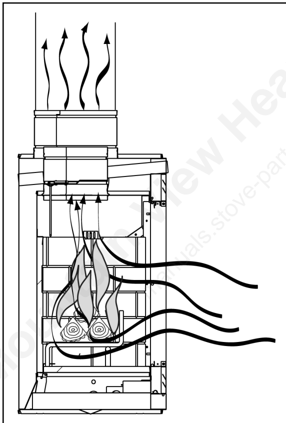
Figure 27 - Flue Draft
