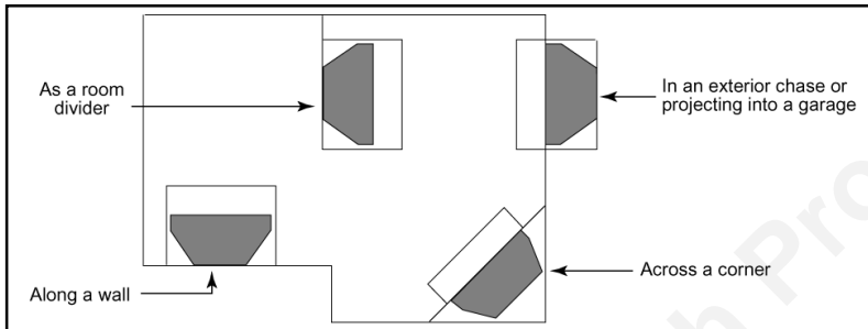
Figure 2 - Fireplace Locations
