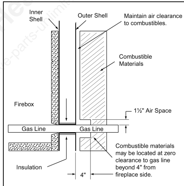
Figure 16 - Air Clearance Around Gas Line
