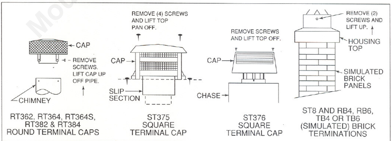
Figure 20 Terminal Caps
