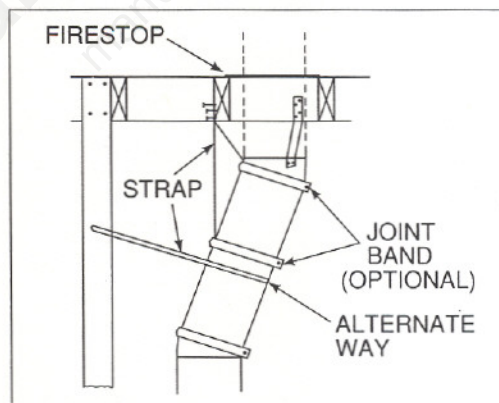
Figure 16 Offset/Return Installation
