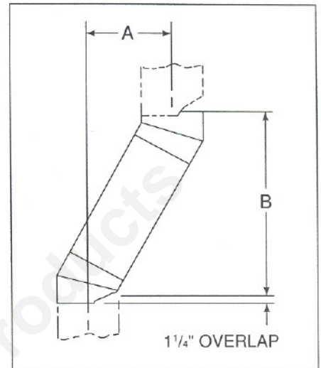
Figure 9 Chimney Offset/Return
