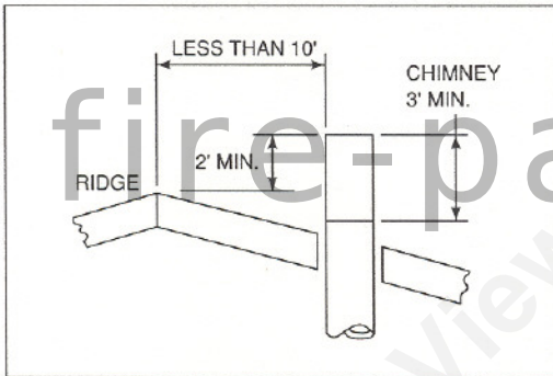
Figure 11 Chimney Height
