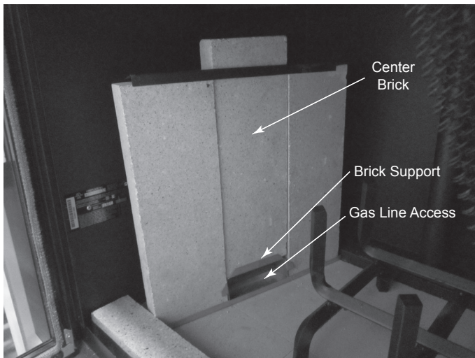
Figure 8.4 Gas Line Installation
