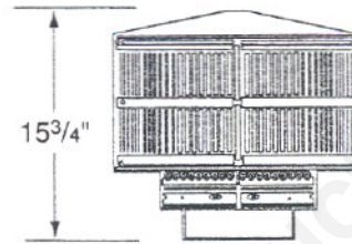
TR344 ROUND TERMINAL CAP WITH STORM COLLAR
