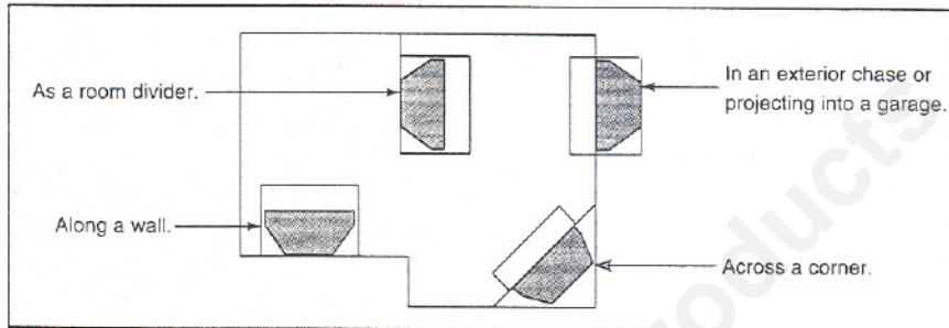
Figure 1 Fireplace Locations
