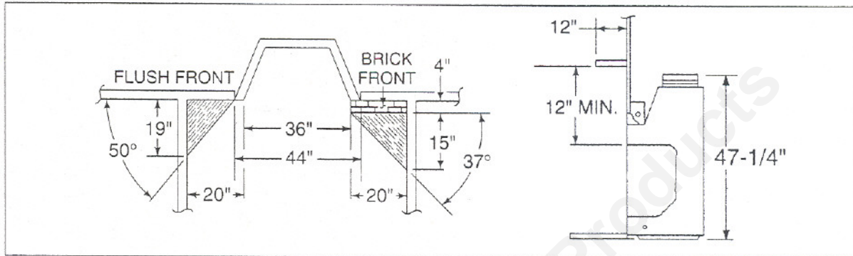
Figure 7 Sidewalls/Surrounds
