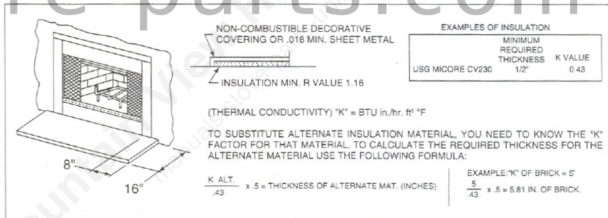
Figure 6 Hearth Extension
