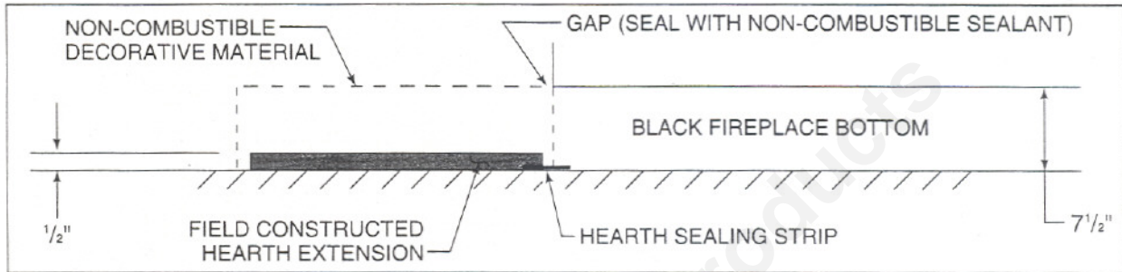
Figure 5 Field Constructed Hearth Extension
