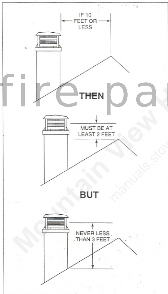
Figure 9 Chimney Height
