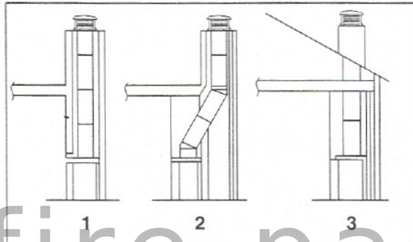
Figure 22 Chase Constructions
