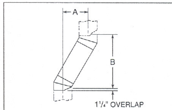
Figure 8 Chimney Offset/Return
