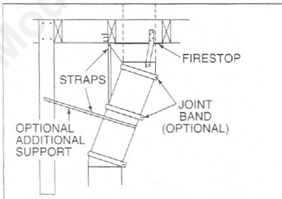
Figure 15 Offset/Return with Stabilizer
