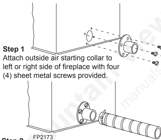
Attach Outside Air Starting Collar to Fireplace Figure 25
