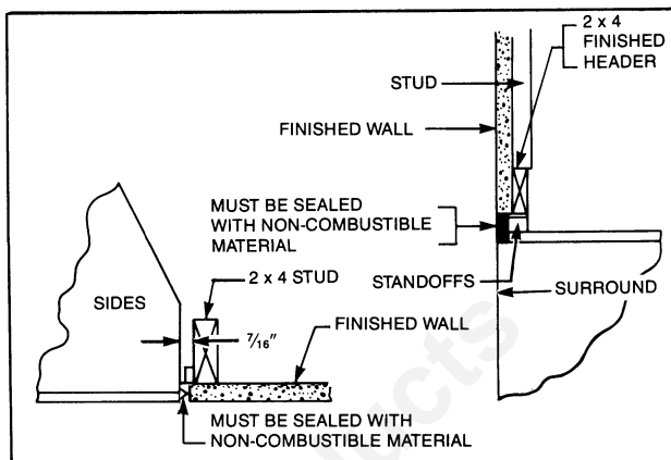
Fig. 21. Fireplace surround flush with finished wall.
