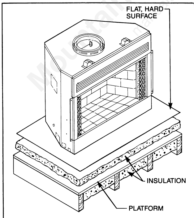
Fig. 17. Insulation between platform and fireplace.
