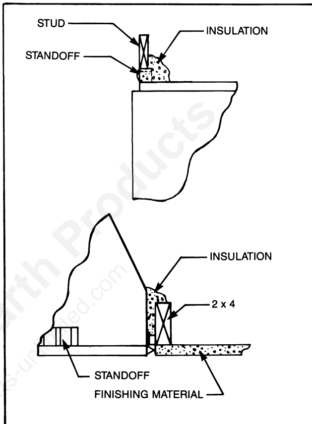
Fig. 18. Sealing spaces between fireplace and finishing materials.
