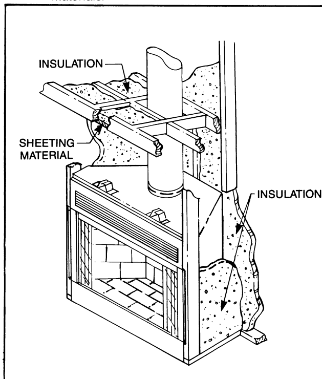
Fig. 19. Additional insulating methods.
