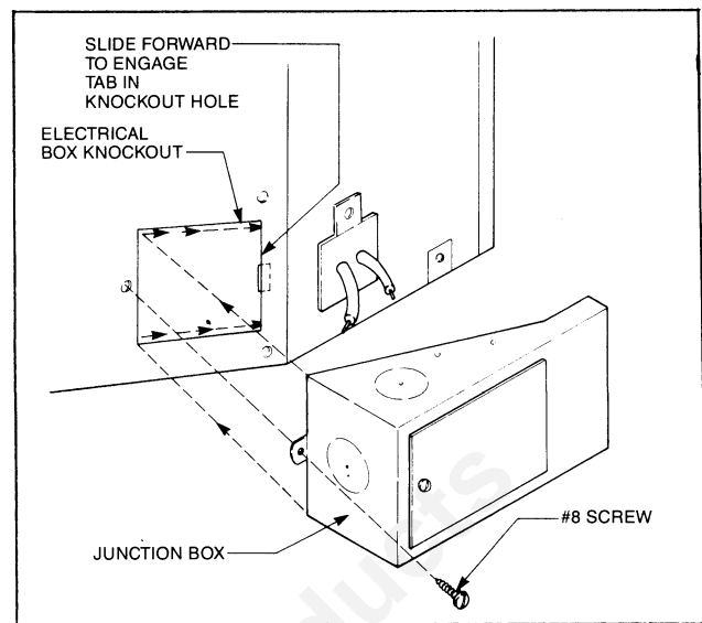
Fig. 14. Wiring box being mounted.
