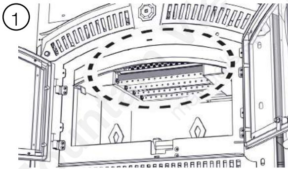
1 Locate the ceramic fibre baffle.
