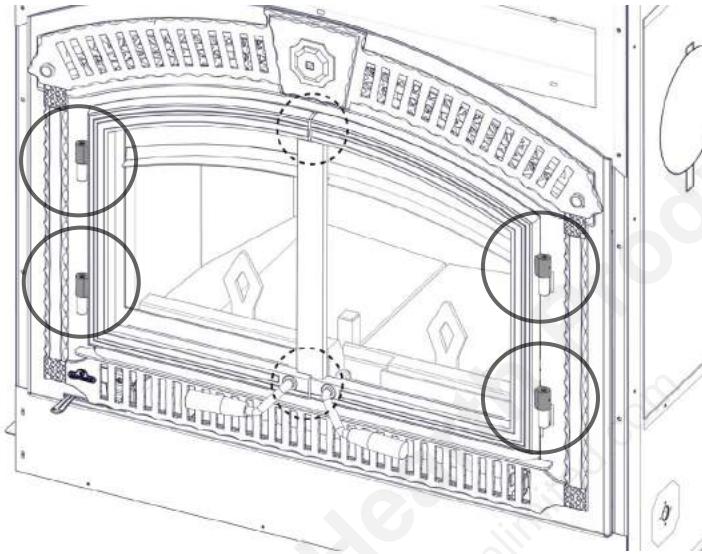
Door gap and hinge location
