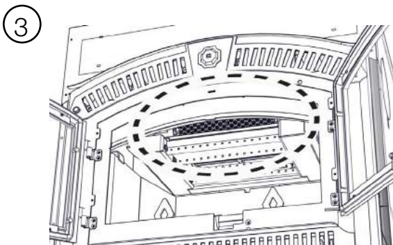
3 Perforated catalyst shield location.
