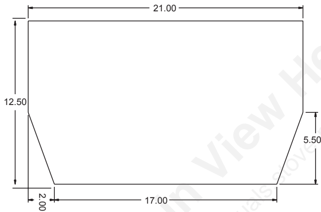
Yosemite 1/2 inch 832-3390
