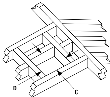
Roof Framing
