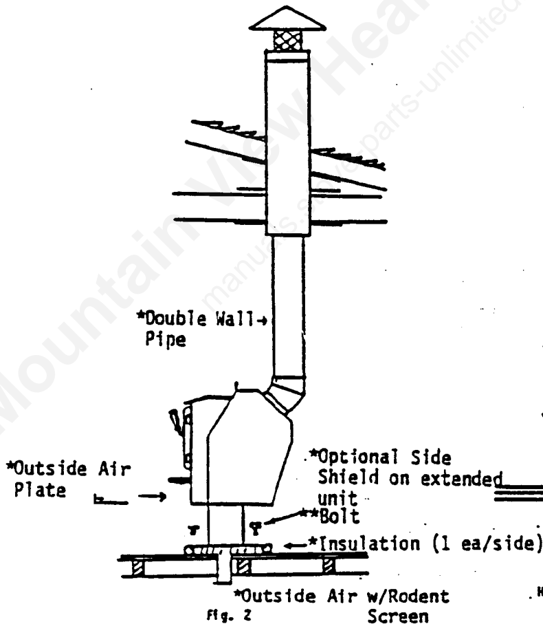
VERTICAL INSTALLATION WITH FACTORY BUILT CHIMNEY
