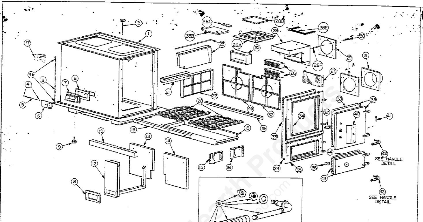
FIGURE 15 - (HEATER REPAIR PARTS. SEE LEDGER ON NEXT PAGE FOR PART NAMES AND PART NUMBERS).
