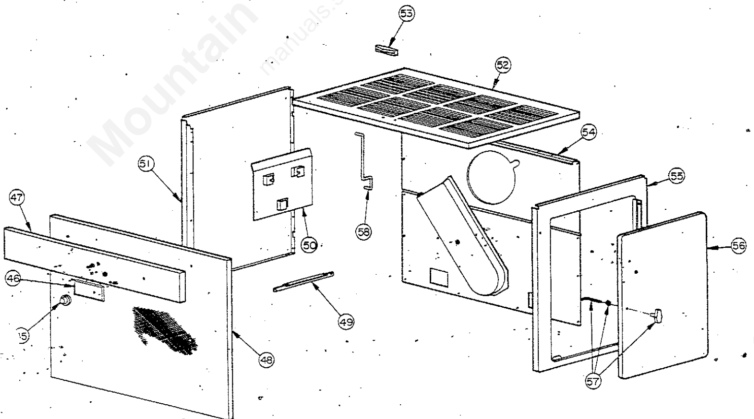
FIGURE 17 -- (HEATER REPAIR PARTS. SEE LEDGER ON NEXT PAGE FOR PART NAMES AND PART NUMBERS).
