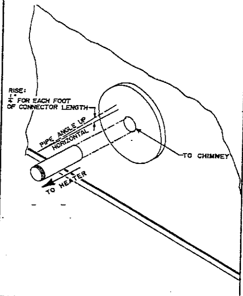
FIGURE 6 - RISE OF HORIZONTAL CHIMNEY CONNECTOR PIPE
