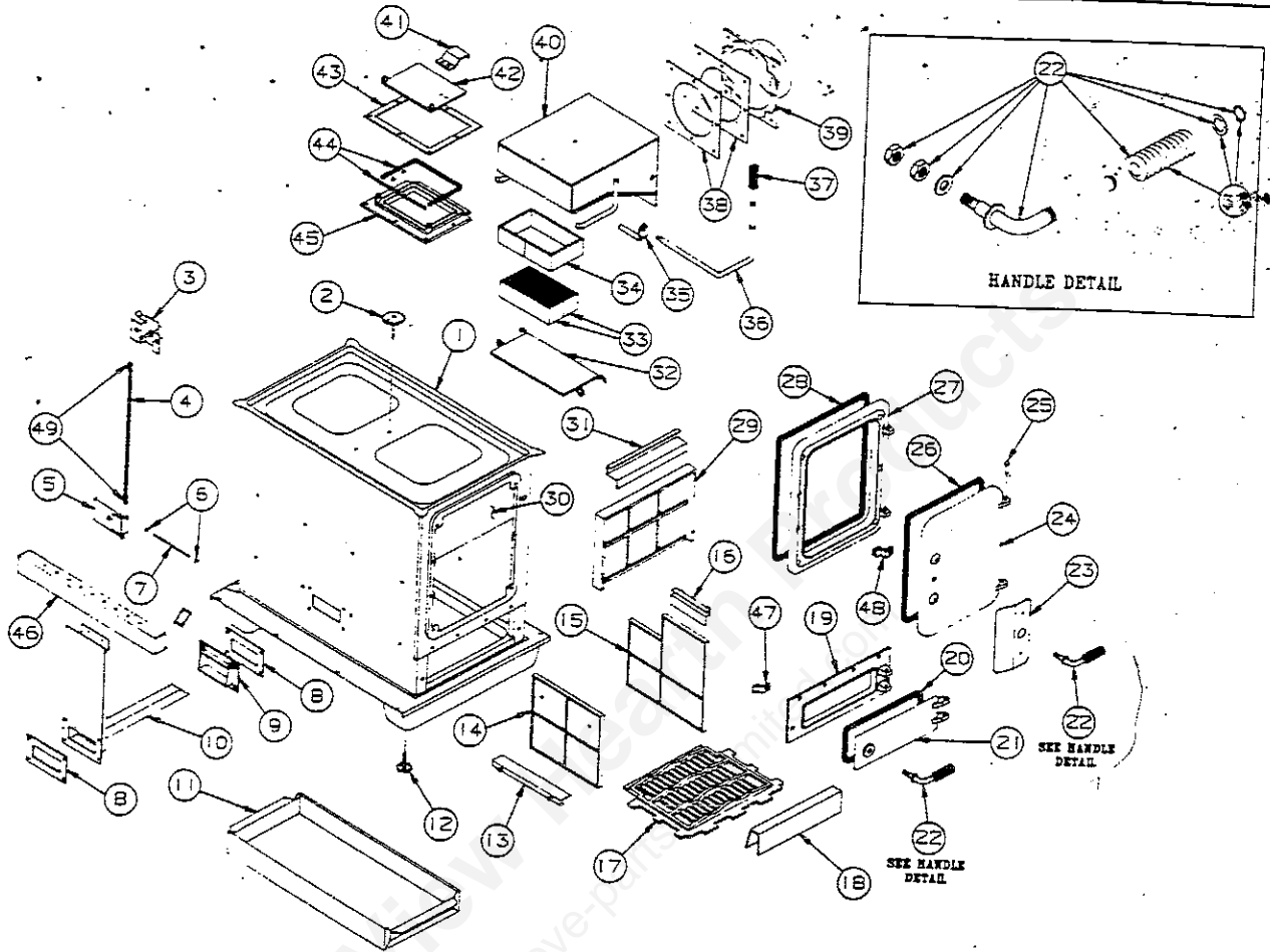
FIGURE 15 -- (HEATER REPAIR PARTS. SEE LEDGER ON NEXT PAGE FOR PART NAMES AND PART NUMBERS).
