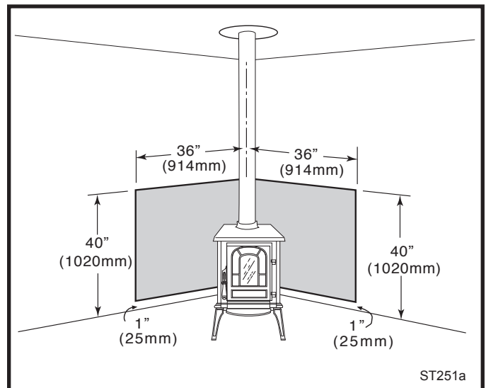
Fig. 19 Corner installation, vertical chimney connector, two wall shields.
