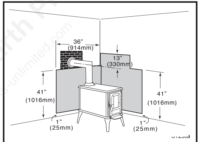
Fig. 18 Parallel installation with rear wall pass-through, two wall shields.
