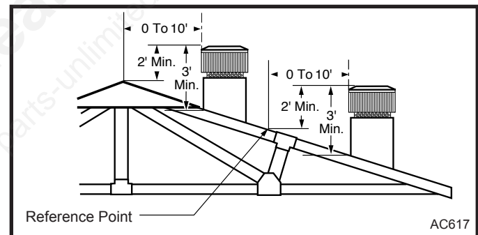
Fig. 2 The 2'-3'-10' Chimney Rule.
