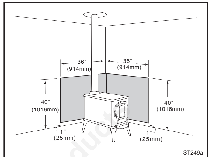
Fig. 17 Parallel installation, vertical chimney connector, two wall shields.
