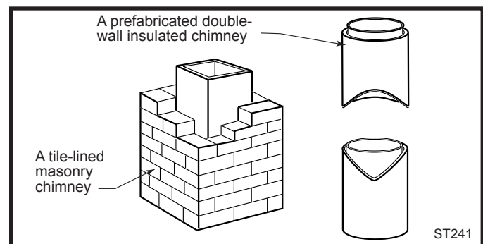
Fig. 3 Standard Chimney Types
