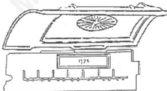
TWO - PIECE FIREBACK WITH CURVED UFB
