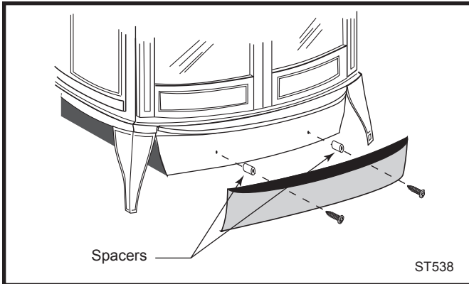
Fig. 24 Install the ashdoor heat shield.
