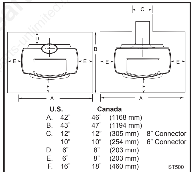
Fig. 12 Required floor protection dimensions.
