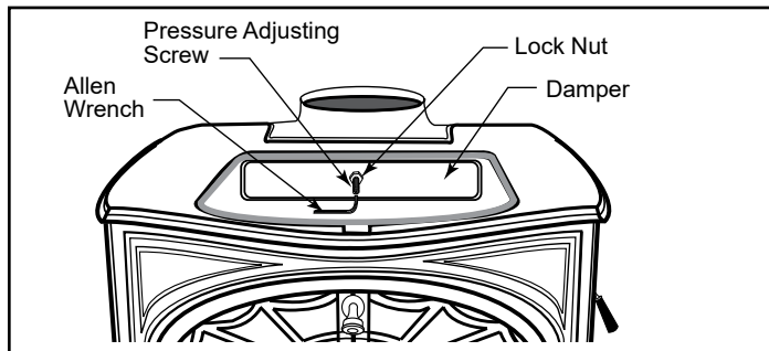
Figure 44 - Adjust the damper with the Allen wrench.
