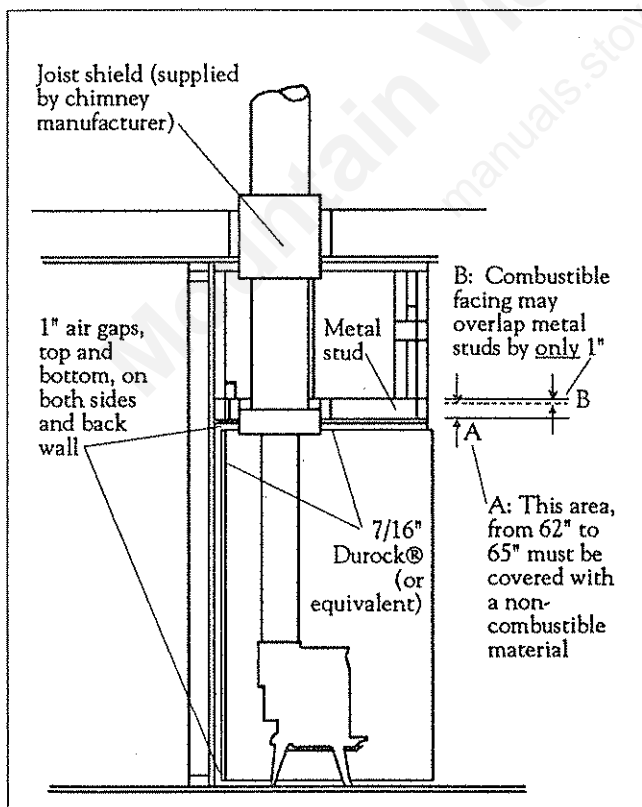
Side section.
