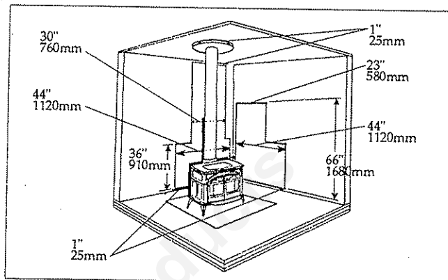
Parallel installation, vertical chimney connector, with stove, connector and wall shields. Maximum reduction for both rear and side walls. Wall shields may meet at corner if desired. A heat shield 24" (610mm) in diameter suspended 1" (25mm) below the ceiling must surround the chimney.
