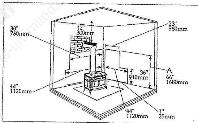
Parallel installation with rear wall pass-through with stove, connector and wall shields. Wall shields may meet at corner if desired. Connector shield extends 28" (710mm) above flue collar, or to the elbow, whichever is less. Height "A" must be 66" (1680mm) or reach the thimble. Pass-through must comply with codes. See "Special Installations".
