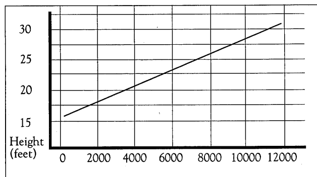
Fig. 1. Chimney height requirements for Encore when equipped with a 6" chimney.
