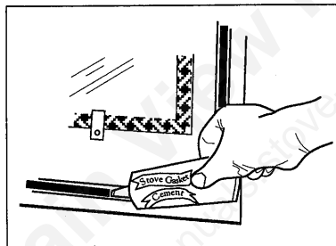
Fig. 57. Apply new cement to the clean channel.
