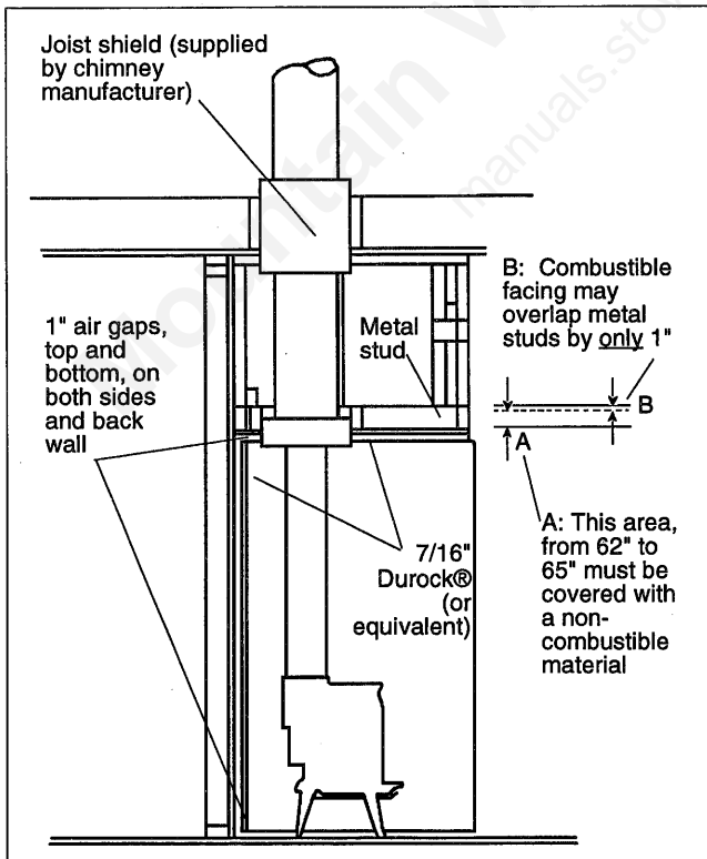
Fig. 18. Side section.
