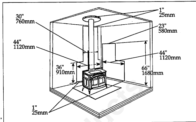
Fig. 23. Parallel installation, vertical chimney connector, with stove, connector and wall shields. Maximum reduction for both rear and side walls. Wall shields may meet at corner if desired. A heat shield 24" (610mm) in diameter suspended 1" (25mm) below the ceiling must surround the chimney.
