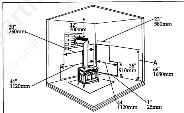
Fig. 25. Parallel installation with rear wall pass-through with stove, chimney connector and wall shields. Wall shields may meet at corner if desired. Connector shield extends 28" (710mm) above flue collar, or to the elbow, whichever is less. Height "A" must be 66" (1680mm) or reach the thimble. Pass-through must comply with codes. See "Special Installations".
