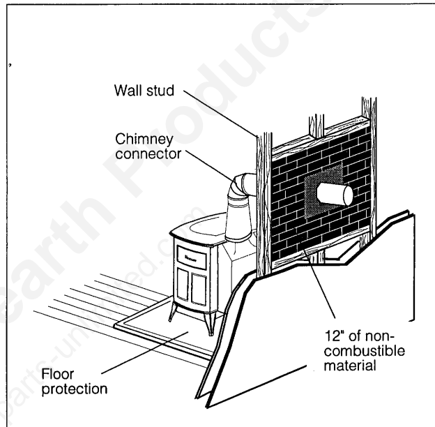
Fig. 9. An approved wall pass-through for the United States.
