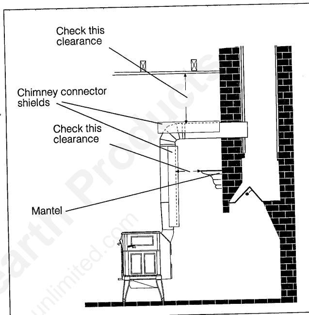
Fig. 7. In this installation, the chimney connector is attached to the chimney above the fireplace opening.
