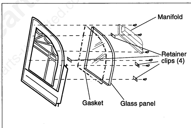
Fig. 44. An exploded view of the glass assembly on the left door.
