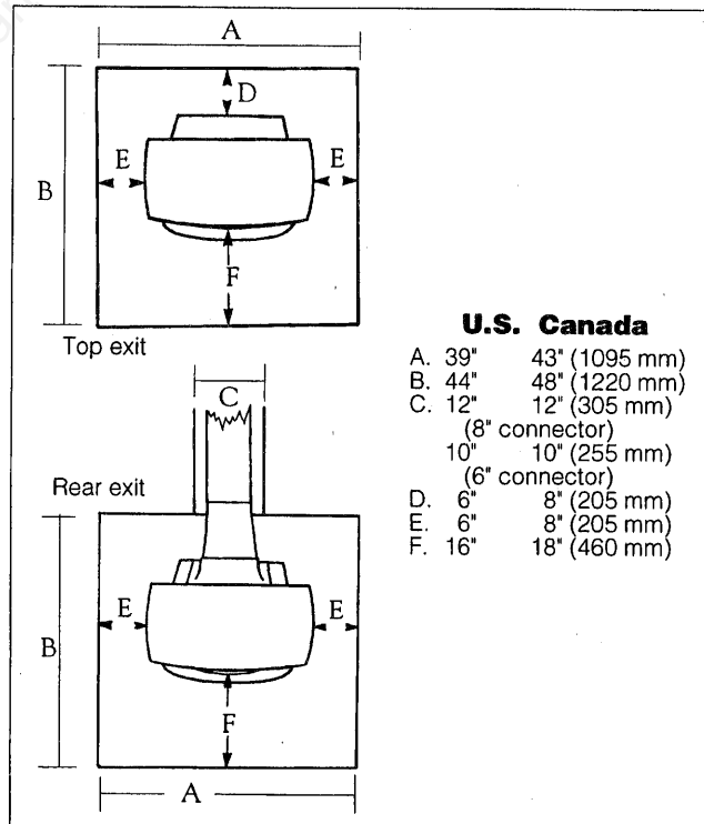
Fig. 11. Required floor protector dimensions for both top- and rear-exiting stoves.
