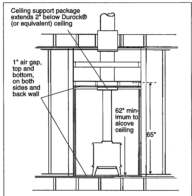
Fig. 21. Front section: 65" minimum clearance from finished floor surface to combustibles on front face. Combustible facing may overlap metal studs by only 1". It should not extend below the height of the non-combustible ceiling.
