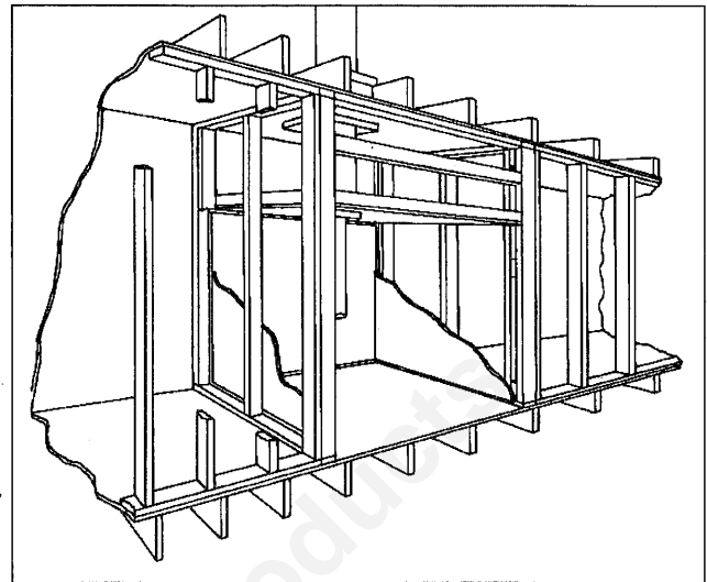
Fig. 19. Cutaway perspective of alcove installation.
