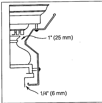
Fig. 15. A custom-formed mantel shield.
