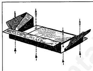
Fig. 29. Use four spacers to attach the bottom heat shield.
