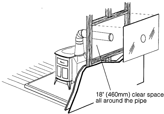
Fig. 10. An approved wall pass-through for Canada.
