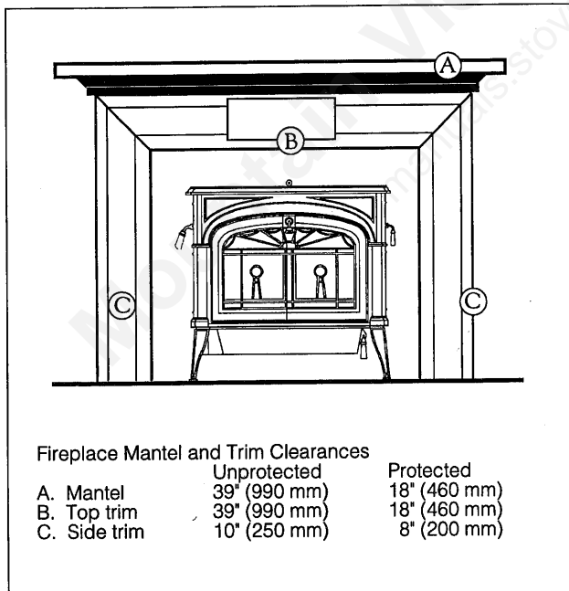
Fig. 16. Maintain clearances to combustible components of the mantelpiece.
