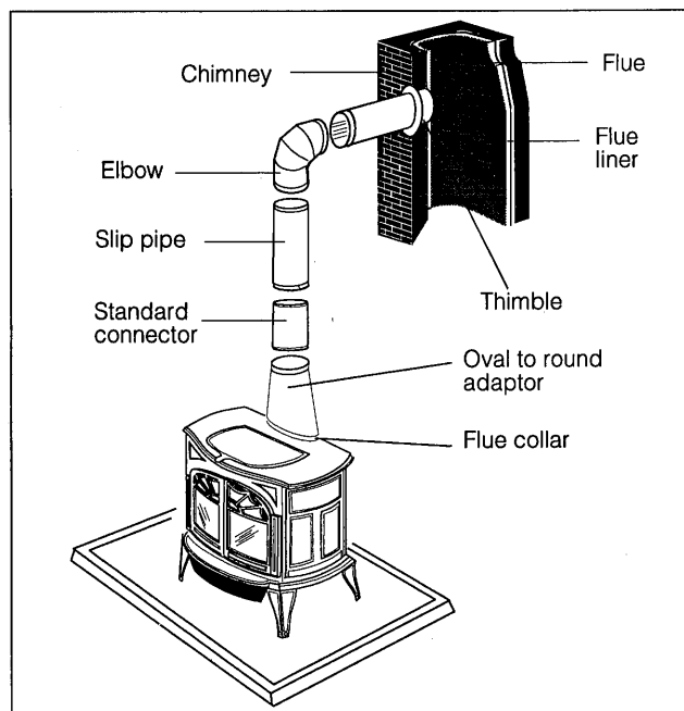
Fig. 5. An exploded view of the chimney connection in a freestanding masonry installation.
