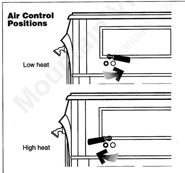
Fig. 33. The handle also may be positioned anywhere between the two extremes for different heat levels.
