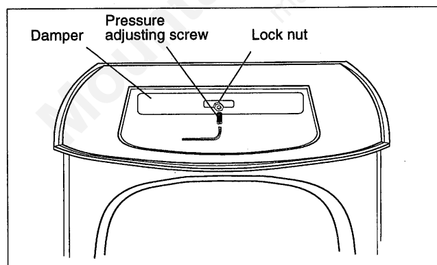
Fig. 46. Adjusting the damper.
