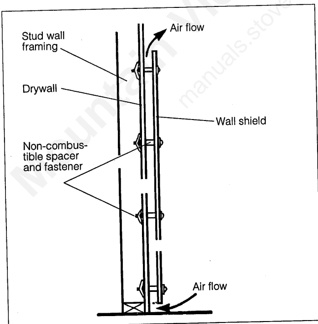
Fig.13. Wall shields must be spaced out from the combustible surface 1" (25 mm) on non-combustible spacers.
