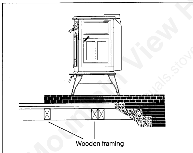
Fig. 12. Combustible supporting timbers may lie beneath fireplace hearths, requiring additional floor protection.
