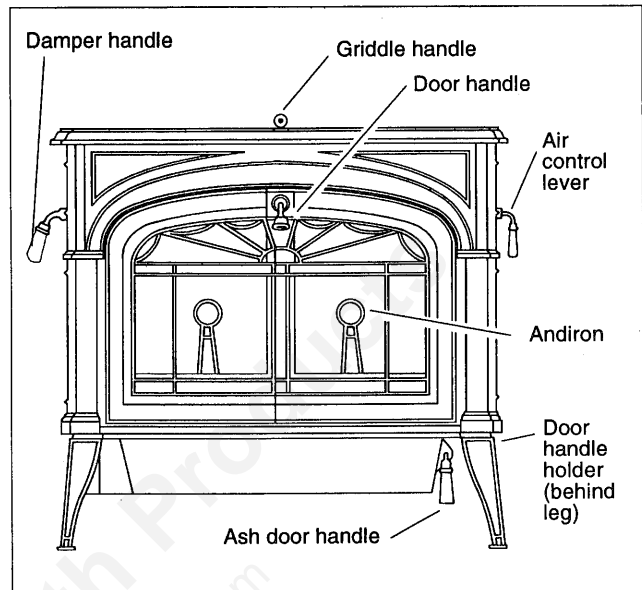
Fig. 34. The Encore controls are conveniently located and easy to operate.
