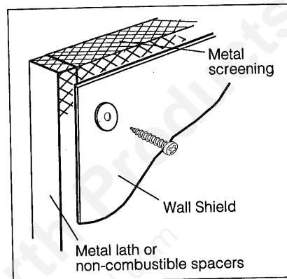
Fig. 14. Metal screening placed over the top of a wall shield will prevent small objects from falling behind it.
