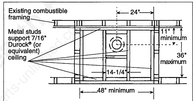
Fig. 20. Reflected ceiling plan.
