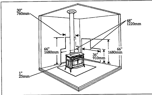
Fig. 22. Parallel installation, vertical chimney connector, two wall shields. Reduced clearances for both rear and side walls. Wall shields may meet at corner if desired. Shielding for connector is centered behind connector.
