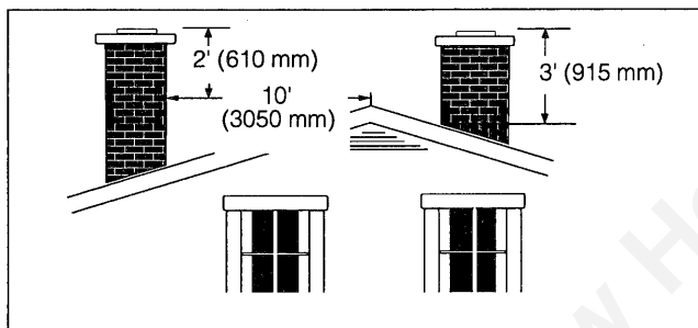
Fig. 3. Observe the 2/3/10 rule for chimneys.
