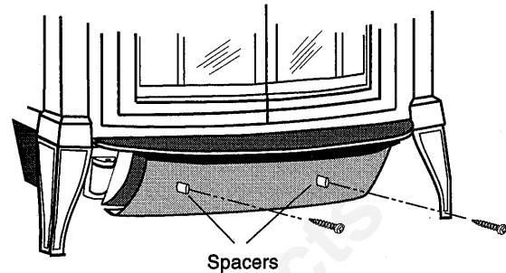
Fig. 30. Use spacers and screws to position the ash door heat shield.
