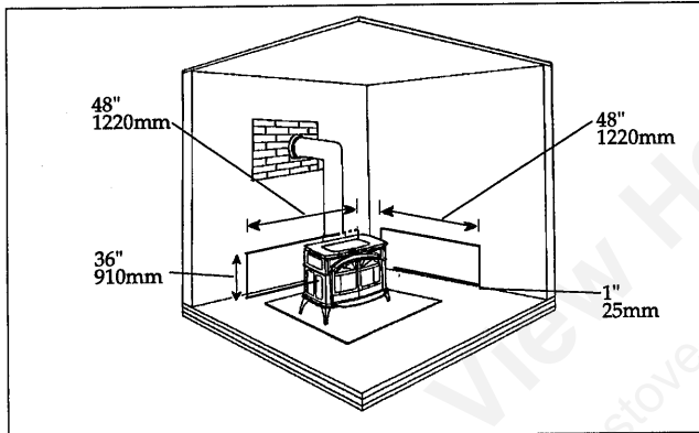
Fig. 24. Parallel installation with rear wall pass-through, two wall shields. Reduced clearances to both rear and side walls. Wall shields may meet at corner if desired. Shielding for connector is centered behind connector. Wall pass-through must comply with codes. See "Special Installations".
