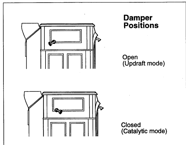
Fig. 35. The damper is either open or closed. There are no intermediate positions.
