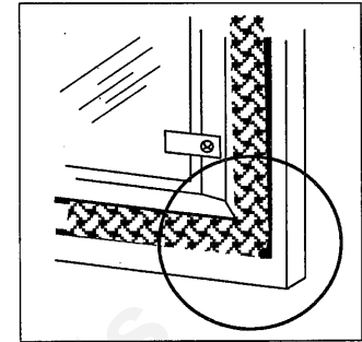
Fig. 59. Seat the gasket in its channel.
