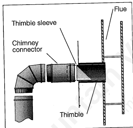
Fig. 6. The thimble, made of either ceramic or metal, must be cemented securely in place.
